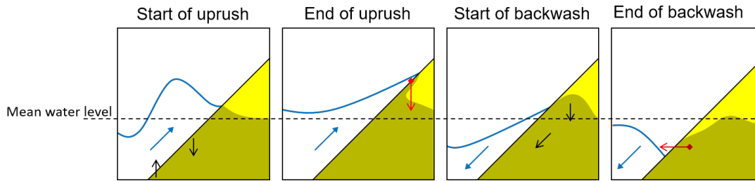
Figure V.5 – Conceptual view of the main flow patterns of beach groundwater induced by swash. Blue lines and arrows are for surface dynamics, black arrows for groundwater dynamics, shaded area depicts the saturated beach and red arrows for infiltration/seepage.
