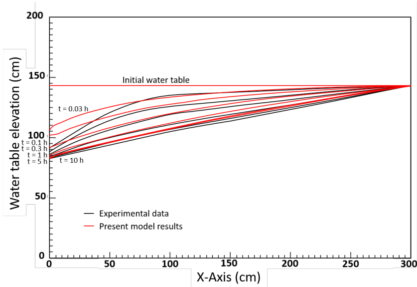
Figure IV.33 – Numerical simulation of two-dimensional drawdown with water table position compared to experimental data from Vauclin et al. [217].
