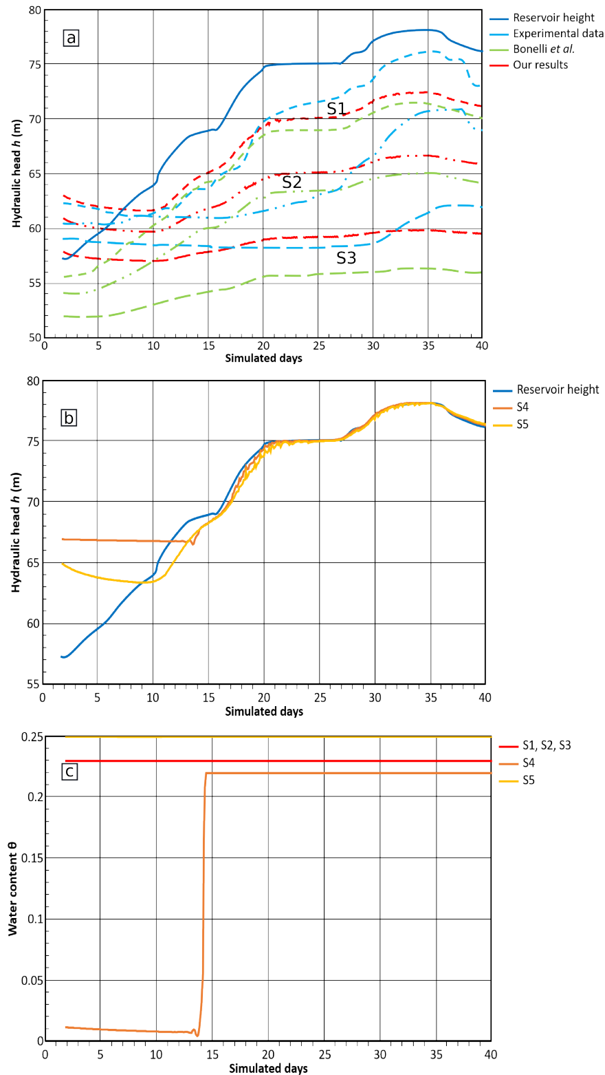
Figure IV.38 – Time evolution of inner dam hydraulic parameters. a) Hydraulic head at sensors S1 (short-dashed lines), S2 (dash-dotted lines) and S3 (long-dashed lines) from the present simulation (red), the experimental data (light blue) and the previous results of Bonelli et al. [91]. The reservoir height is depicted in dark solid line. b) Hydraulic head at numerical sensors S4 (orange) and S5 (yellow). c) Water content at S1 to S5 sensors (note that S1, S2 and S3 show similar values).
