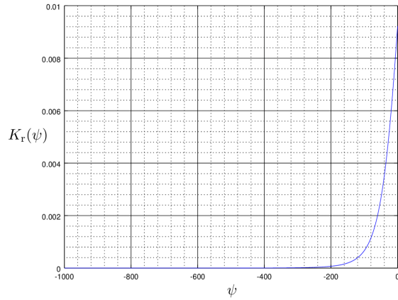
(b) Relative hydraulic conductivity K_r in function of pressure head \psi
