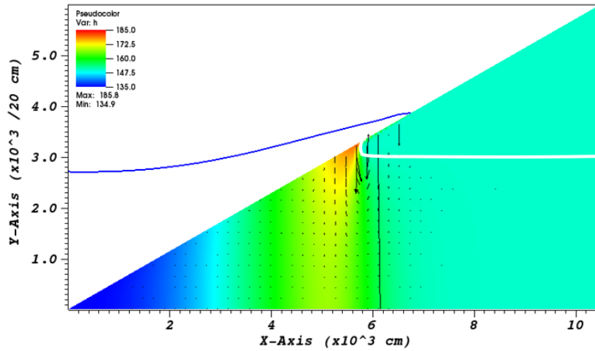
Figure V.8 – Snapshot of hydraulic head contours at t = 37.5 s for the end of the first uprush. Velocities range from about 0.3 to 0.6 cm/h in the beach. Maximum velocity is 35 cm/h for infiltration.
