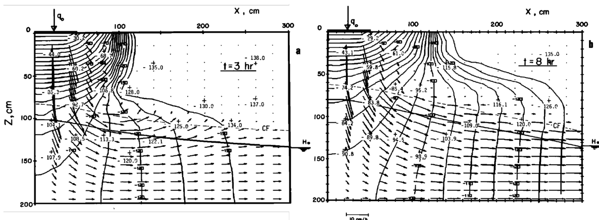
Figure IV.27 – Numerical results from Vauclin et al. [220] for the distribution of hydraulic head and flux, the location of water table (solid line) and capillary fringe (dotted line) at t = 3\text{ h} (top) and t = 8\text{ h} (bottom). The numbers with crosses represent experimental data of hydraulic head (cm). After Vauclin et al. [220].
