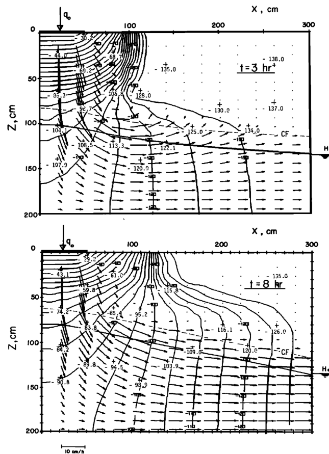
Figure IV.27 – Numerical results from Vauclin et al. [222] for the distribution of hydraulic head and flux, the location of water table (solid line) and capillary fringe (dotted line) at t = 3 h (top) and t = 8 h (bottom). The numbers with crosses represent experimental data of hydraulic head (cm). After Vauclin et al. [222].
