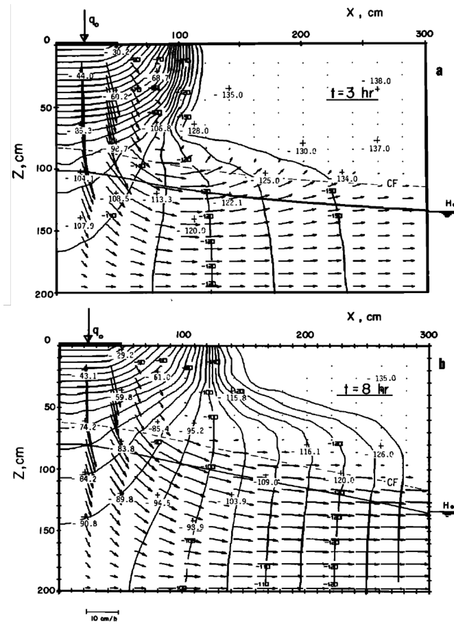
Figure IV.27 – Numerical distribution of hydraulic head (experimental data are numbers with crosses) and flux expressed in centimetres of water. After Vauclin et al. [222].
