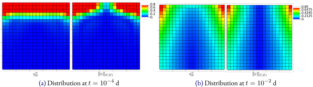
Figure IV.20 – Comparison between distributions of true error in energy norm and the indicator \eta_E^n on Tracy's benchmark.
