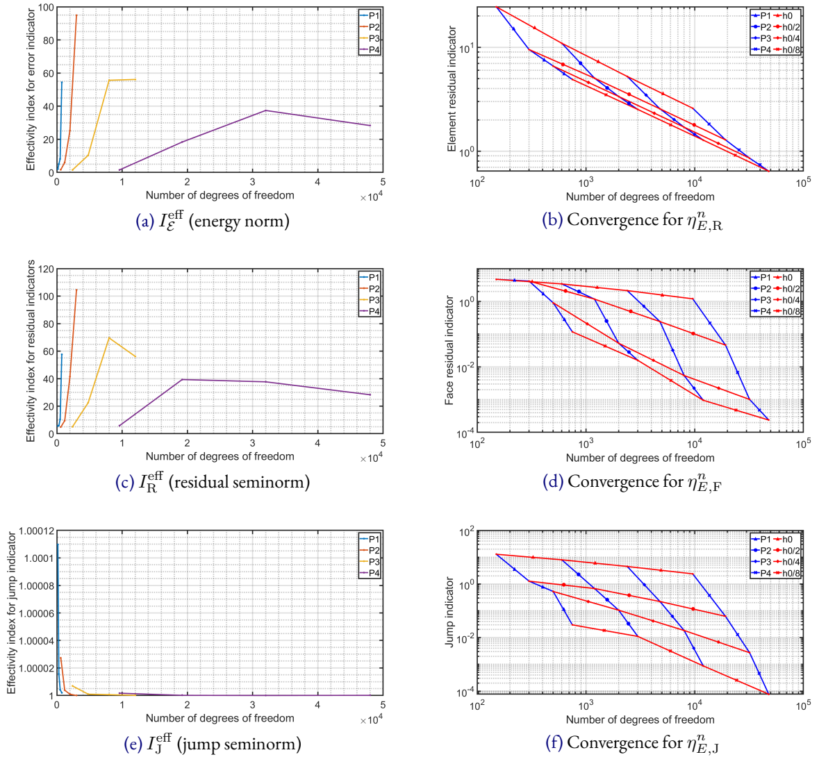
Figure IV.18 – Effectivity indices for different indicators (left) and convergence diagrams for the three parts of the indicator \eta_E^n (right). P1, P2, P3 and P4 stands respectively for linear, quadratic, cubic and quartic approximations.
