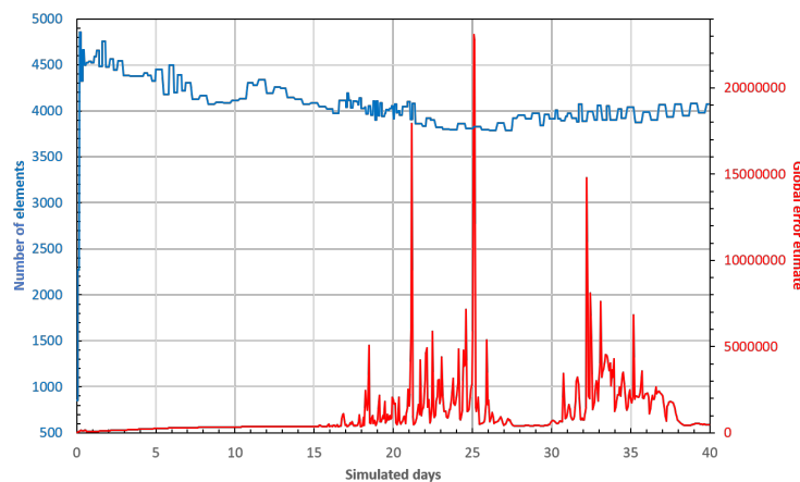
(b) Number of elements and global estimate evolution
