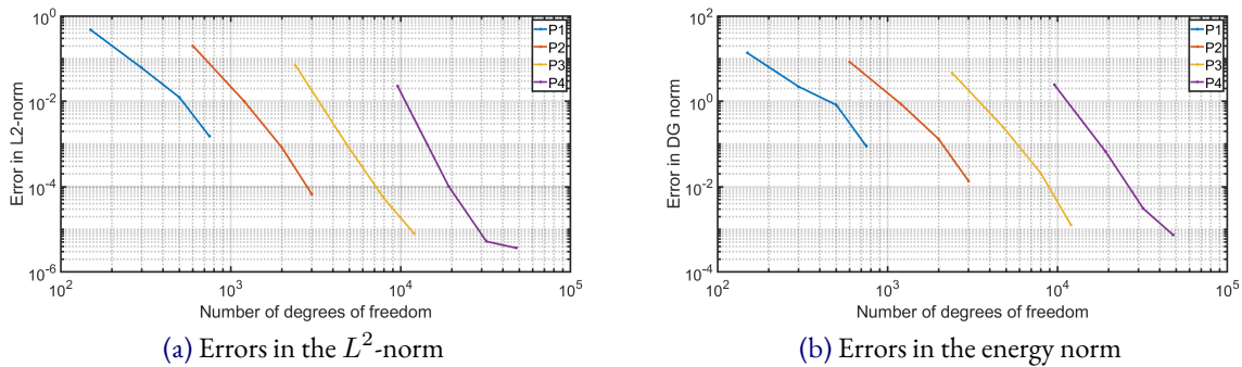
Figure IV.17 – Numerical convergence for Tracy's benchmark. P1, P2, P3 and P4 stands respectively for linear, quadratic, cubic and quartic approximations.
