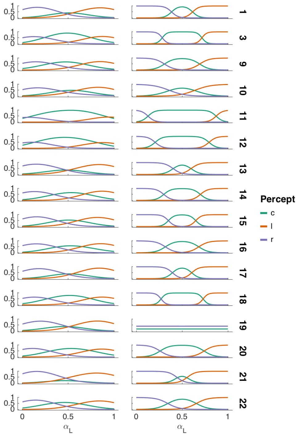
Figure 4.17. Empirical data & model. Left column , the p(\alpha_L|X) (normalised) densities using the empirical probability density estimation method. Right column , the p(X|\alpha_L) using the observer model after estimating \Theta for each participant over the 200 short trial data set, using the post-hoc approach. Subject numbers are listed on each row.
