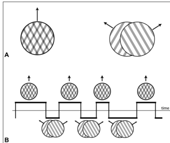
Figure 4.3. Moving plaid perception. Diagrams presenting the perceptual dynamics of the multi-stable moving plaid stimulus. A: diagram showing the two different perceptual interpretation considered in the case of the bi-stable plaid. B: diagram showing a schematic example of the temporal discourse of perception. Figure taken from (Rubin, Hupé, et al., 2005).
