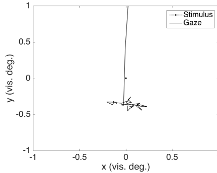
(c) Example of a simulated micro-saccade with GraFEM.
