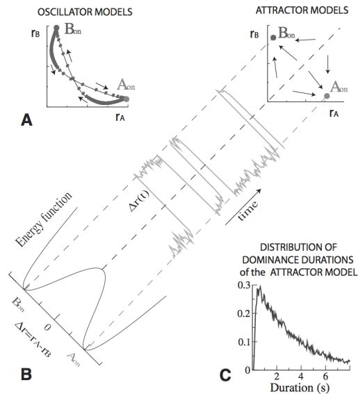
(a) Diagrams comparing oscillator and attractor models.
