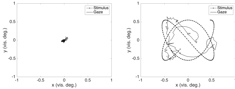
(a) Example of a simulated fixation with (b) Example of a simulated micro-pursuit with GraFEM.
