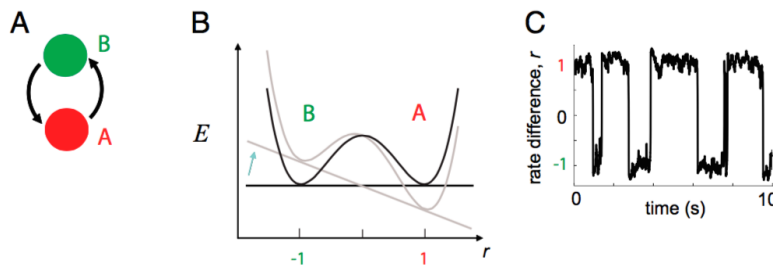
(b) Bi-stable model.
