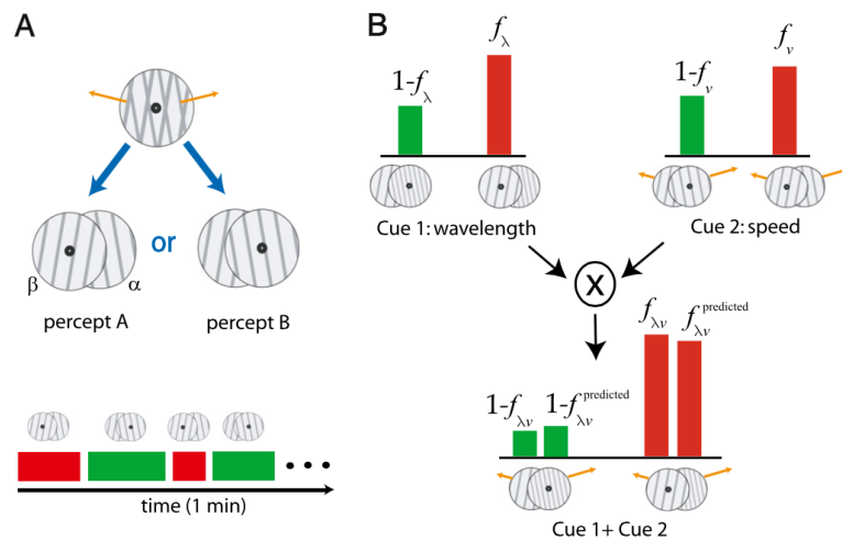
(a) Bi-stable moving plaid.
