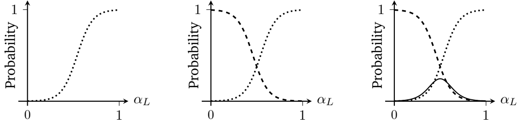
Figure 4.13. Model construction. Diagram showing the composition of the psycho-observer model. On the left, the Sigmoid function for the X = l percept, see Equation (4.14). At the centre, the model when adding the X = r percept using the hypothesis of symmetry between transparency percepts. On the right, the full model when adding the X = c percept using the hypothesis of complementarity of the 3 percepts.
