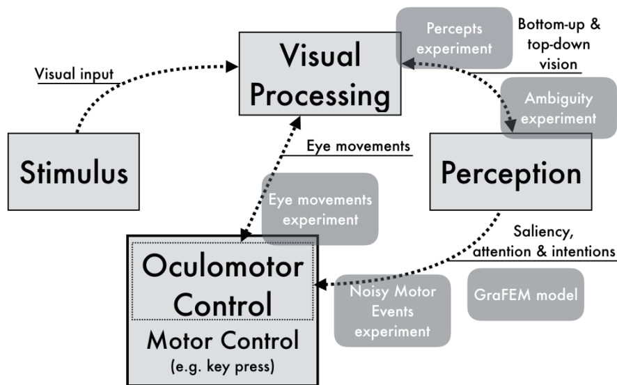
Figure 4.6. Active multi-stable perception. Diagram showing a simplified representation of the motor and perceptual systems, and their interactions for visual perception. The experiments listed are placed as they test specific interactions when observing a multi-stable moving plaid stimulus.
