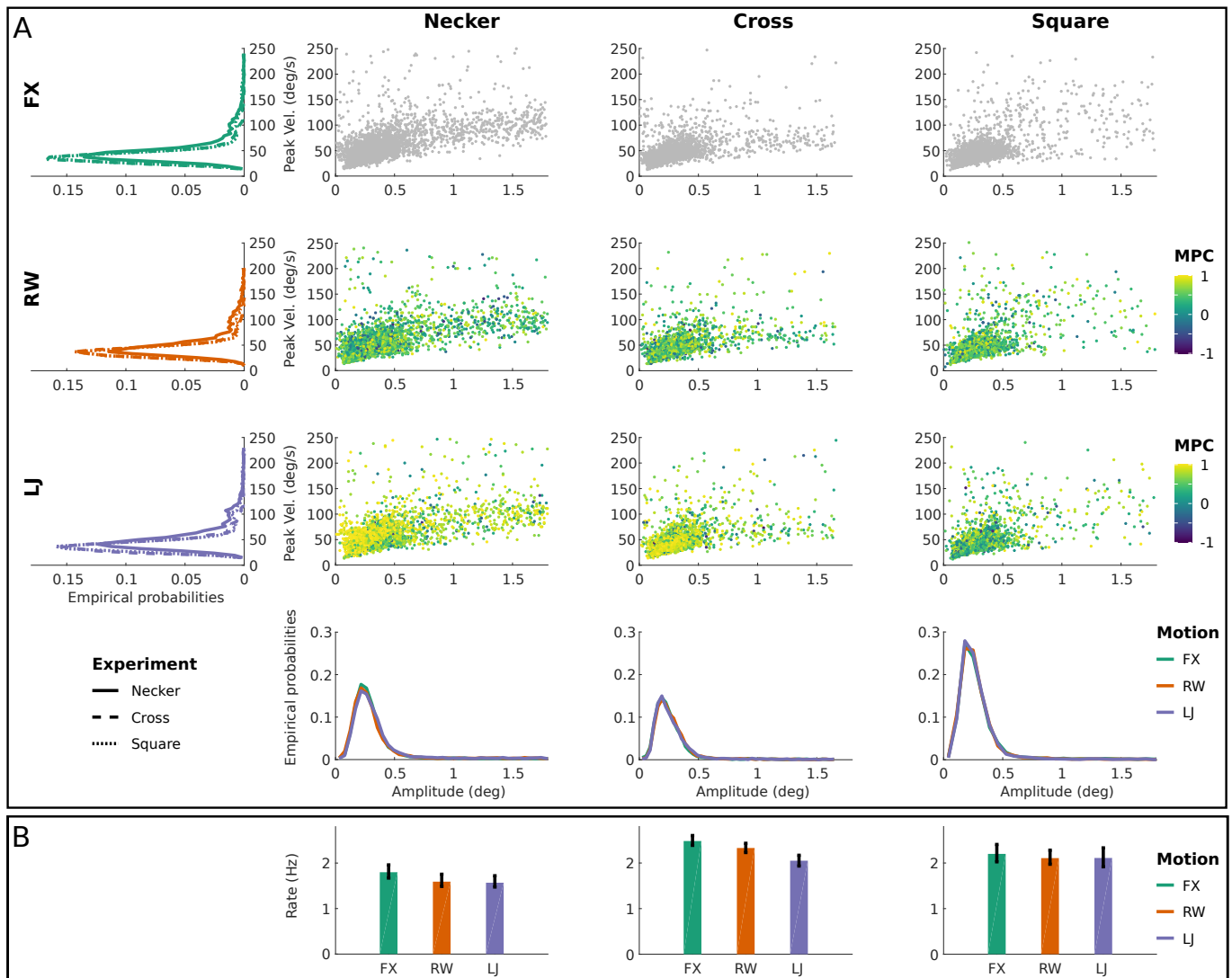
Figure 2: Micro-saccade analysis. A shows the main sequences when plotting micro-saccades' amplitudes versus peak velocities for all three experiments (Necker, Cross and Square) and conditions (FX, RW, LJ). The color encodes the micro-saccade's fixation similarity score (using MPC) in the LJ and RW conditions. Left side , marginal distributions of peak velocity depending on the experiment and condition are given, while below , marginal distributions for amplitudes are shown. B shows mean micro-saccade rates over experiments and conditions with, in black, 95% confidence intervals computed using bootstrap ( n = 200 iterations).
