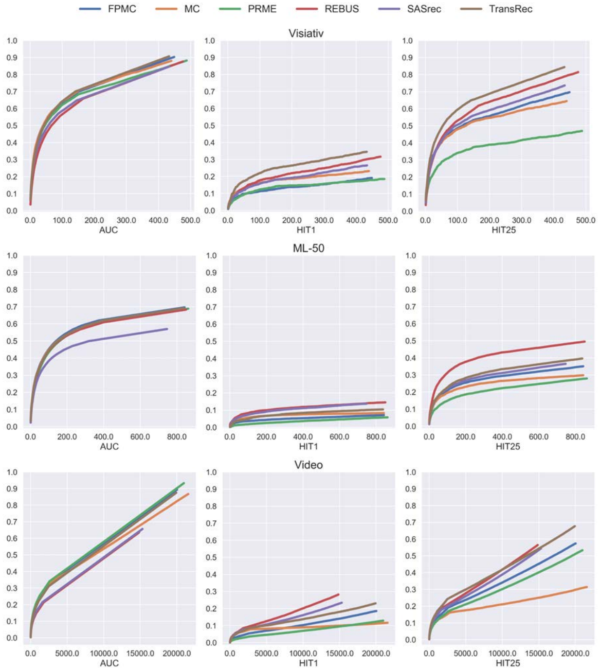
Figure 4.12: AUC, HIT1 and HIT25 values with respect to the number of SDD patterns selected to build the global explanation related to a recommendation model for Visiativ (first row), ML-50 (second row) and Video (last row) datasets. The higher the value, the higher the fidelity of the global explanation to the black box recommender model.
