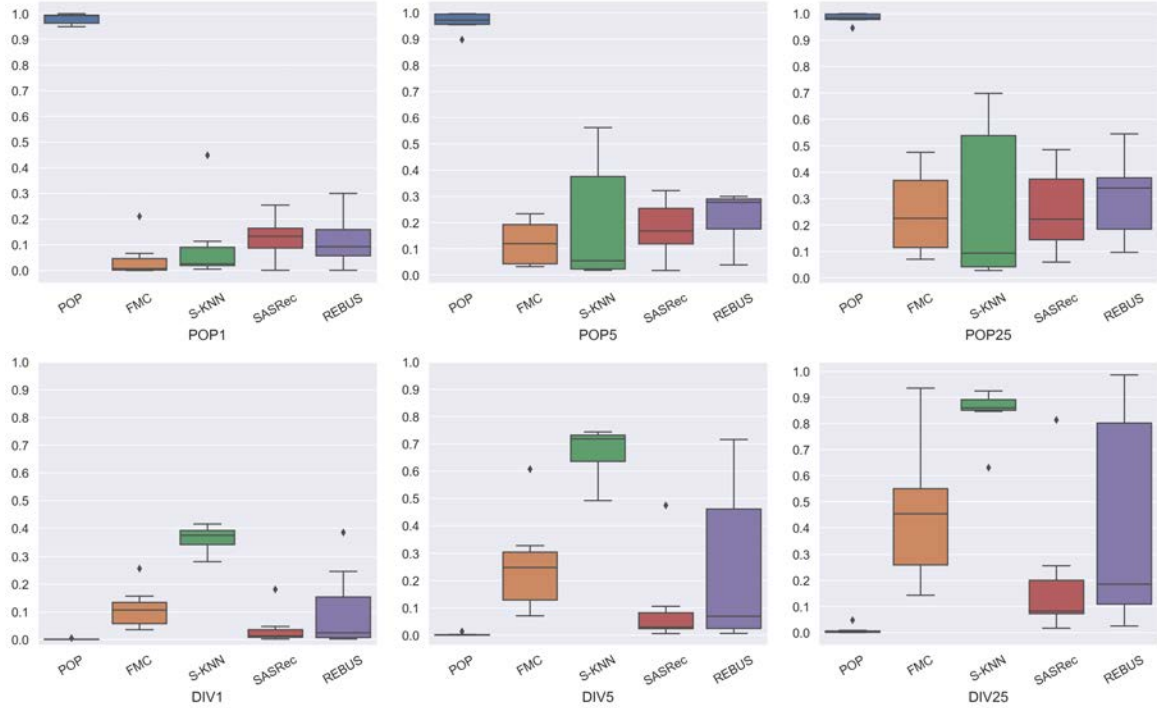
Figure 3.4: Performance of POP _X (first row) and DIV _X (second row) with X \in \{1, 5, 25\} for the different models that do not suffer of the problem of cold-start users. Values are averaged over all datasets.
