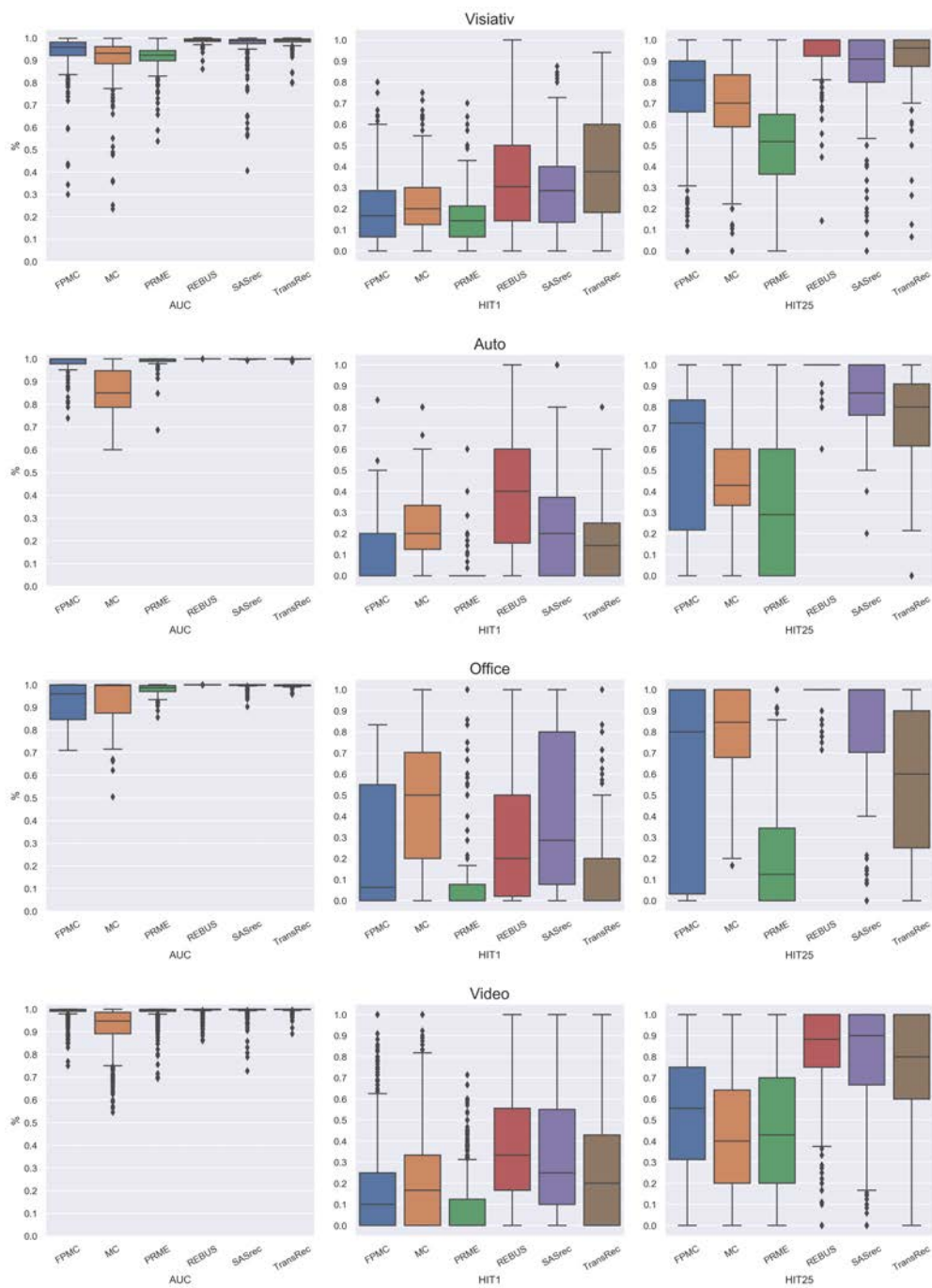
Figure 7.3: Performance metrics for Visiativ and Amazon dataset (AUC, HIT1 and HIT25) evaluated on SDD subgroups descriptions found in at least 6 users for each model.
