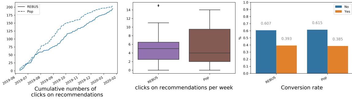
Figure 5.8: Evolution of the cumulative number of clicks on recommendations (left), number of clicks on recommendations per week (center) and conversion rate of clicks to downloads (right) for A/B Test 1 .
