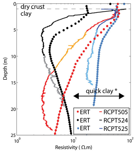
Fig. 4. In situ resistivity logs acquired during three RCPT sounding in Smørgrav quick clay site. Lighter colors depict measurements where the clay was characterized as “quick” by RPS investigations. The local quick clay resistivities are slightly lower than the established range of 10–80 Ω·m (*, Solberg et al., 2012). Three vertical logs (dots) extracted from the constrained BERT2 model are plotted for comparison.
