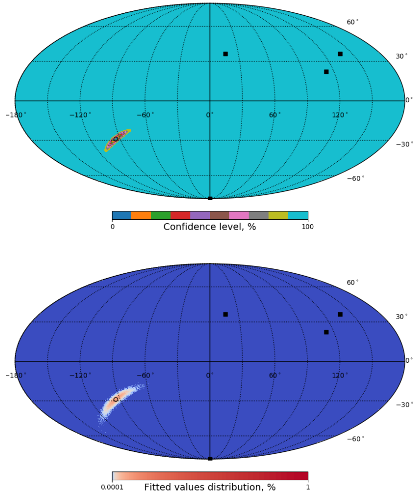
Figure 4.35: Mollweide projection of confidence area in equatorial coordinates for a CCSN at the Galactic Centre (black dot) computed using triangulation between four detectors (black squares): IceCube, KM3NeT/ARCA, Hyper-Kamiokande and JUNO. Top: confidence area assuming true delays, bottom: fitted positions distribution for 100000 realisations of the delay sets [252]
