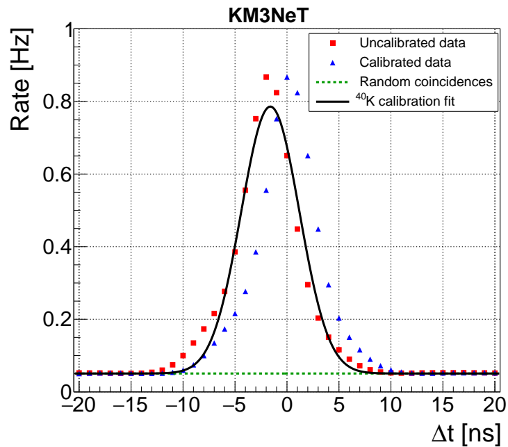
Figure 2.10: Distribution of the time differences between the hit in coincidences for a pair of near-by PMTs for uncalibrated (red) and calibrated (blue) hit times. Superimposed are the calibration fit (black) and the background of random coincidences (green) with uniformly distributed time differences. Source: [163].
