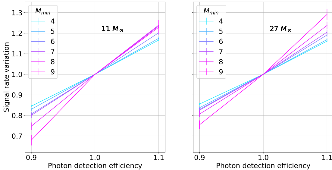
Figure 4.8: Relative variation of the number of detected coincidences with a given minimum multiplicity as a function of the relative variation of the PMT photon detection efficiency used in the simulation. On the left for the 11 M_{\odot} model and on the right for the 27 M_{\odot} model.
