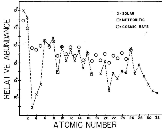
Figure 1.3: Comparison of the relative abundances of the elements in the cosmic radiation at the top of the Earth’s atmosphere, and in the solar photosphere (except for the meteoritic values for F and Cl). Solar data are normalized to hydrogen ( 10^{12} ); cosmic ray data are normalized so that the abundances of carbon coincides with that of Solar carbon. Source: [6].
