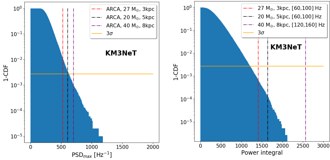
Figure 4.33: Complementary background CDF built from an ARCA noise simulation (blue distribution). On the left as a function of the maximum power. On the right as a function of the power integral around the SASI frequency predicted by the model. The horizontal line (orange) indicates the 3\sigma threshold for the CDF. The vertical lines, dashed red, black and purple correspond respectively to the expectation for the signal plus background scenarios for the 27M_{\odot} , 20M_{\odot} , 40M_{\odot} progenitors at 3, 5 and 8 kpc.
