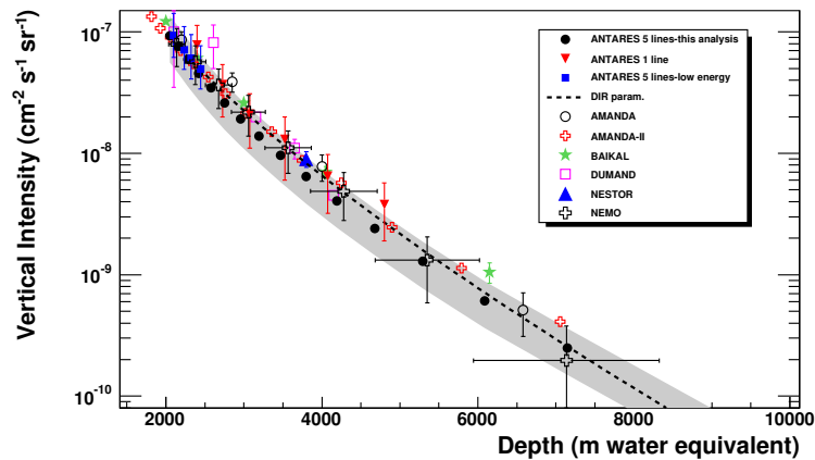
Figure 1.29: Vertical muon flux of atmospheric muons for the 5 line ANTARES data (black points) as a function of the slant depth. Downward triangles show the results from line 1 data. Full squares show the results obtained with a new method and a low muon energy event selection [147]. Expectation from Bugaev parametrization (dotted line) is superimposed [148]. A compilation of results obtained with other underwater detectors is shown: AMANDA, AMANDA-II, Baikal, DUMAND, NESTOR, NEMO.
