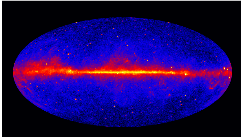
Figure 1.13: Fermi-LAT 60-month image, constructed from front-converting \gamma -rays with energies above 1 GeV. The most prominent feature is the bright band of diffuse glow along the map's center, in correspondence of the Galactic Plane. Credits: NASA / DOE / Fermi-LAT , svs.gsfc.nasa.gov/11342 .
