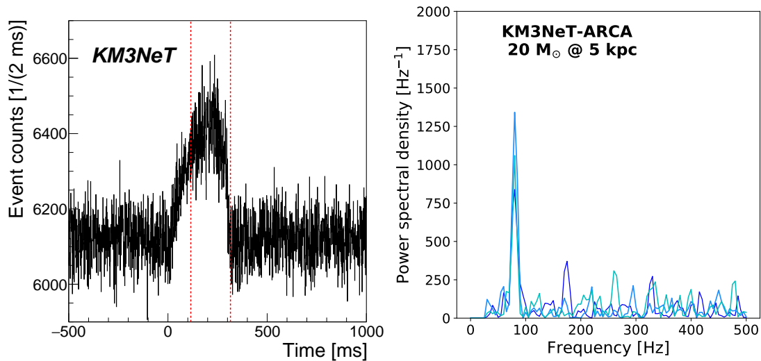
Figure 4.32: Left: simulation of a neutrino light-curve for all coincidences at multiplicity two and above detected for a 20M_{\odot} progenitor in an ARCA building block. Right: power spectrum as calculated for different realisations of the signal simulation.
