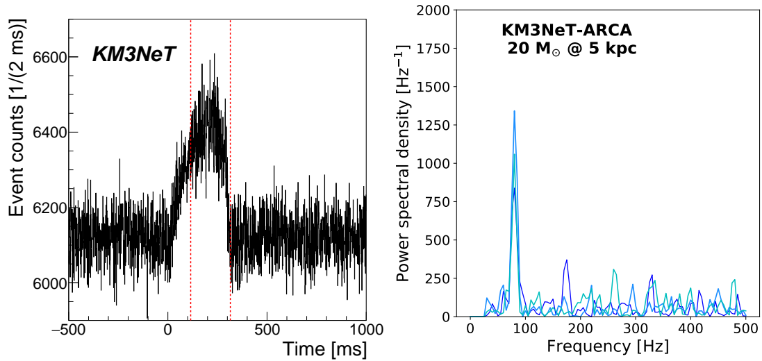
Figure 4.32 – Left: simulation of a neutrino light-curve for all coincidences at multiplicity two and above detected for a 20 M_{\odot} progenitor in an ARCA building block. Right: power spectrum as calculated for different realisations of the signal simulation.
