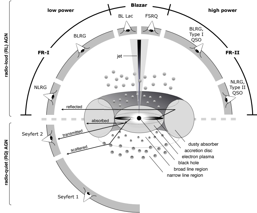
Figure 1.16 – Schematic representation of AGN classification [94]. The type of visible object depends on the viewing angle, on the jet and the power of the central engine. Radio loud object are thought to have symmetric jets. Author: Marie-Luise Menzel (MPE). Source: [95].
