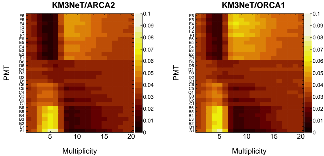
Figure 3.9 – Probability of the PMT contribution to coincidence rates as a function of the multiplicity (each abscissa bin is normalised to unity). The PMT is identified by the ring (letter) and the position of the PMT on the ring (number). The first address (A1) refers to the vertical down-facing PMT, rings from B to D belong to the lower hemisphere, while rings E and F belong to the upper hemisphere of the DOM (see Figure 3.4). Above a multiplicity of 20, statistical fluctuations dominate the pattern, and are therefore left out of the figure. Author's work published in [163].
