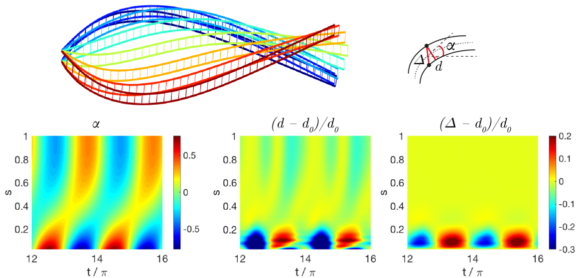
Figure 7.7 – Coupling between two filaments obtained with the coarse-grained approach. Here \text{Sp} = 4 , a = 0.88 rad, K/\kappa = 1/25 . On the top, the actuated filament is represented at regular intervals of time over half a time period, coloured from blue (beginning) to red (end). The three colormaps display three parameters with respect to time and arclength: the angle \alpha of the centerline (left), the distance d between the two filaments (middle) and the distance \Delta between two facing nodes, normalised by their resting length d_0 . Note that the beginning time for the graphs has been chosen big enough to skip transient phase and display only steady state. A travelling wave of curvature generated by the actuation of the top filament is visible in graph at the bottom left. The graph at the bottom in the middle shows the distance between the two filaments. Moreover, the graph at the bottom right captures the sliding distance between the two filaments.
