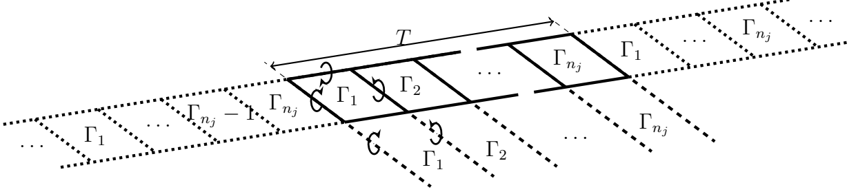
Figure 5.2 – Infinite wing Vortex Lattice Method with periodicity assumption.
