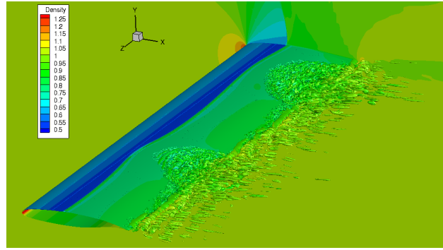
Figure 3.4 – Q-criterion iso-surface of level 60.0 colored by density and density contour on the plane z/c = 4 and the wing surface.
