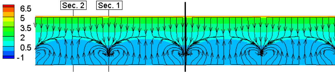
Figure 2.21 – Surface pressure coefficient and skin friction lines with 224 (left) and 112 (right) spanwise cells ( \alpha = 15.0 deg.).
