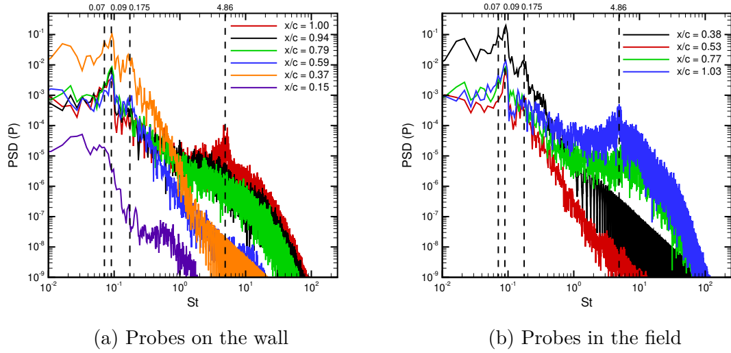
Figure 3.6 – Power spectral density of the pressure in the large span ZDES simulation.
