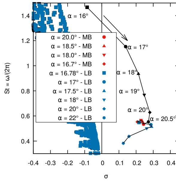
Figure B.4 – Effect of the angle of attack on the spectra of the 2-D unstable mode (NACA4412, M = 0.2 , Re = 350\,000 , \delta = 0.0^\circ , \beta = 0 ).
