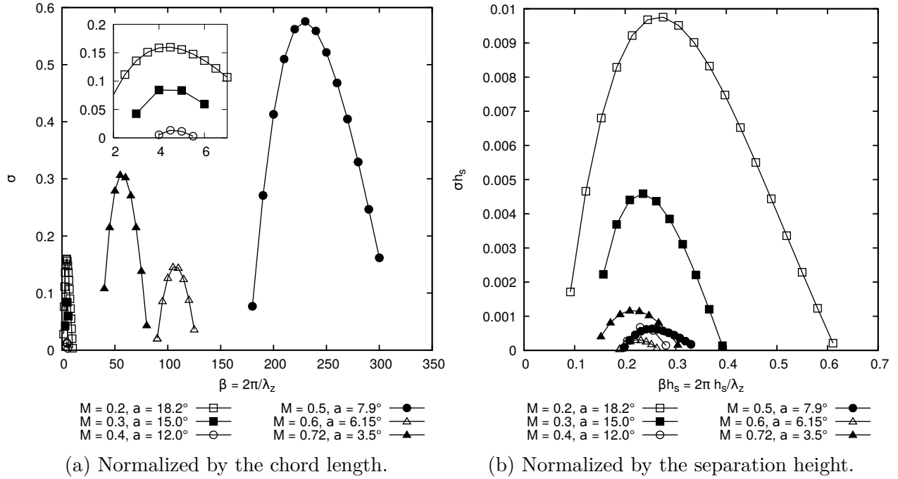
Figure 4.31 – Effect of the Mach number and angle of attack on the growth rate of the 3-D mode (NACA0012, Re = 10^7 , \delta = 0^\circ ).
