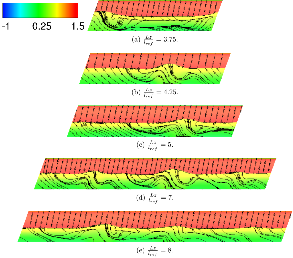
Figure 2.8 – Wing span effect on the number of buffet cells for a sweep angle of 20 deg.
