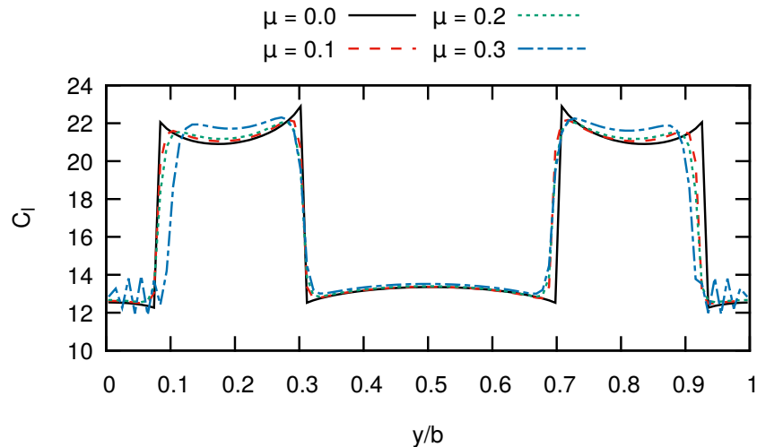
Figure 5.27 – Effect of the artificial dissipation on the effective angle distribution (infinite wing, AR = 2.0 ).
