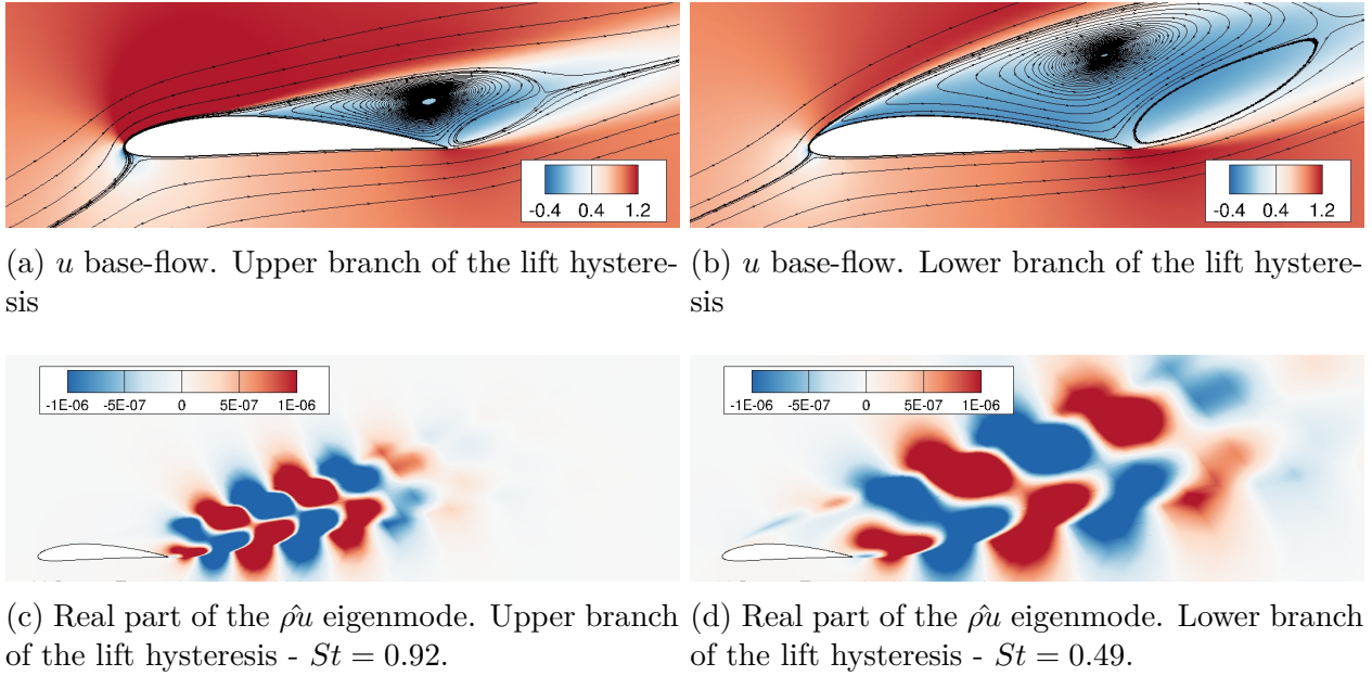
Figure 4.19 – Flow visualisation of the (a,b): base-flow and (c,d): 2-D unstable mode on the two branches of the lift hysteresis (NACA4412, M = 0.2 , Re = 350\,000 , \alpha = 18.0^\circ , \delta = 0.0^\circ , \beta = 0.0 ).
