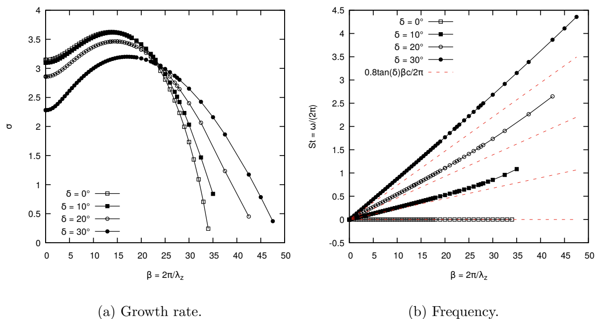
Figure B.7 – Effect of the sweep angle on the growth rate and frequency of the 3-D unstable mode (NACA4412, M = 0.2 , Re = 350\,000 , \alpha = 18.0^\circ , middle branch, black: stability analysis, red: URANS simulations ( \alpha = 15.0^\circ )).
