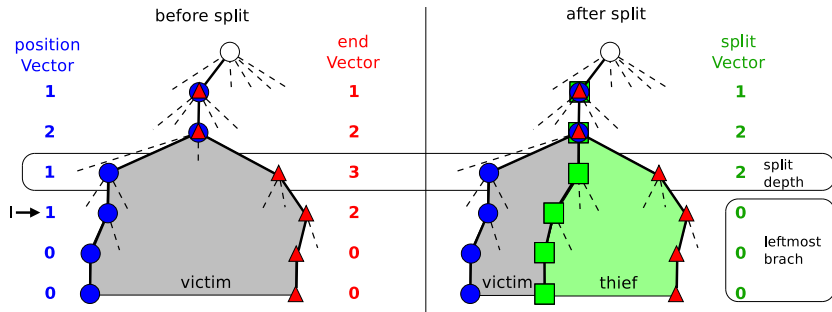
(a) Arithmetic interval splitting
