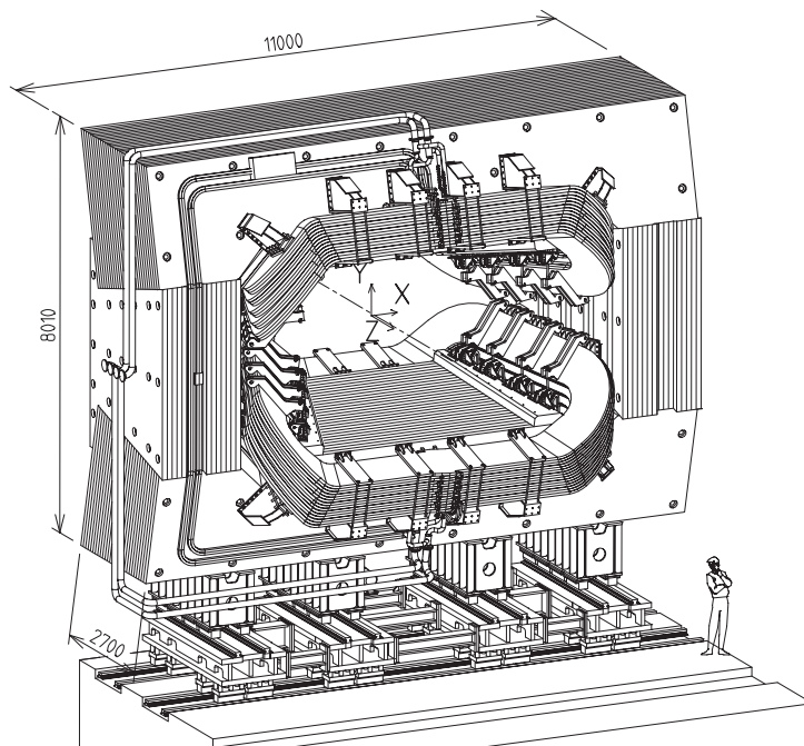
Figure 2.6 – A schematic of the bending dipole magnet projected onto the x - y plane.
