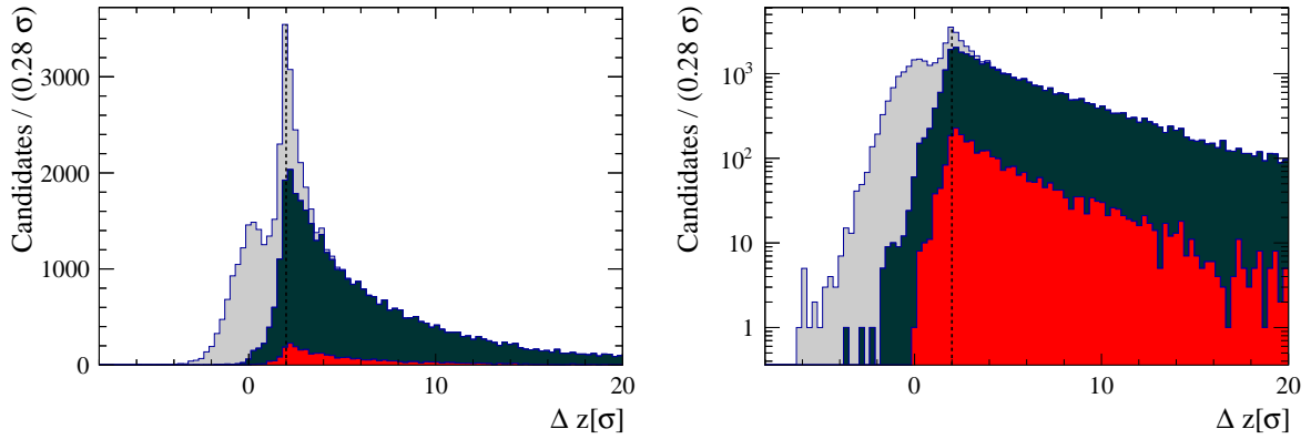
Figure 5.2 – \Delta z/\text{uncertainty} distribution in linear (left) and logarithmic (right) scale of the simulated signal (red), double charm background (black) and prompt background (grey), after the initial cuts except the last three lines of the Table 5.3. A cut at 2\sigma is shown.
