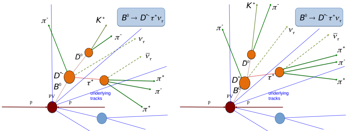
Figure 4.1 – Illustration of two B^0 \rightarrow D^{*+} \tau^+ \nu_\tau ( \tau^+ \rightarrow 3\pi^\pm \bar{\nu}_\tau ) events as simulated in one ReDecay block. Note that the vertices and tracks of the signal mode differ, while the underlying event remains the same.
