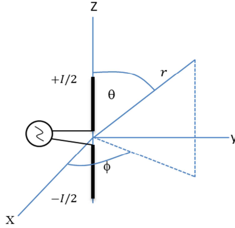
Figure 3.2: The center-fed short dipole antenna with its radiating coordinates.
