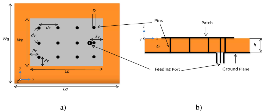
Figure 5.14: Pin loaded single patch antenna: a) top view, b) side view.
