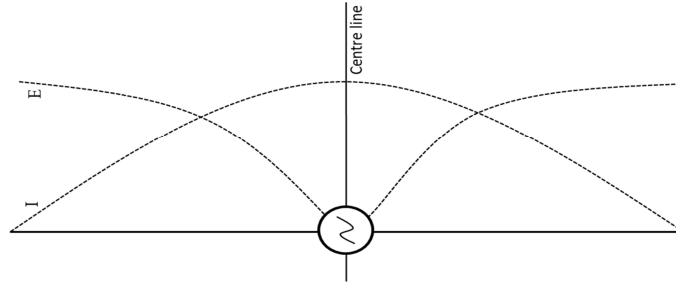
Figure 3.6: Voltage(E) and current(I) relationship in center fed resonant half wavelength wire antenna.
