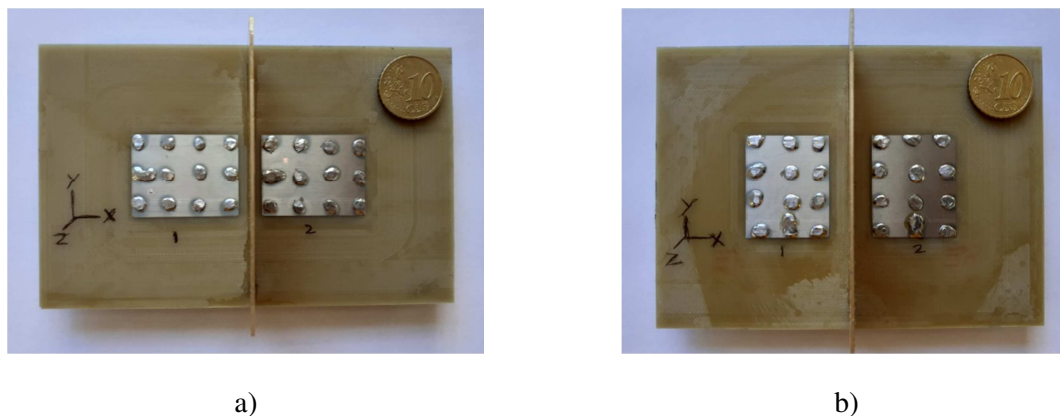
Figure 5.29: Fabricated Pin loaded two element antenna arrays with metallic wall barrier oriented along: a) E-plane, b) H-plane.
