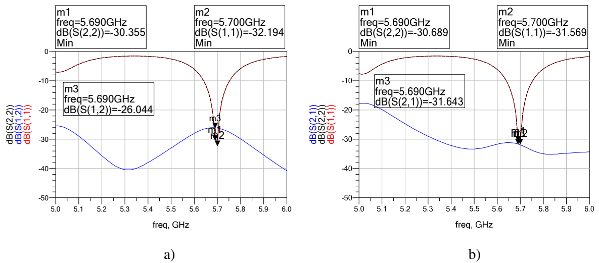
Figure 5.24: Simulated S-parameters of pin loaded two antennas through 3D simulation oriented along: a) E-plane, b) H-plane.
