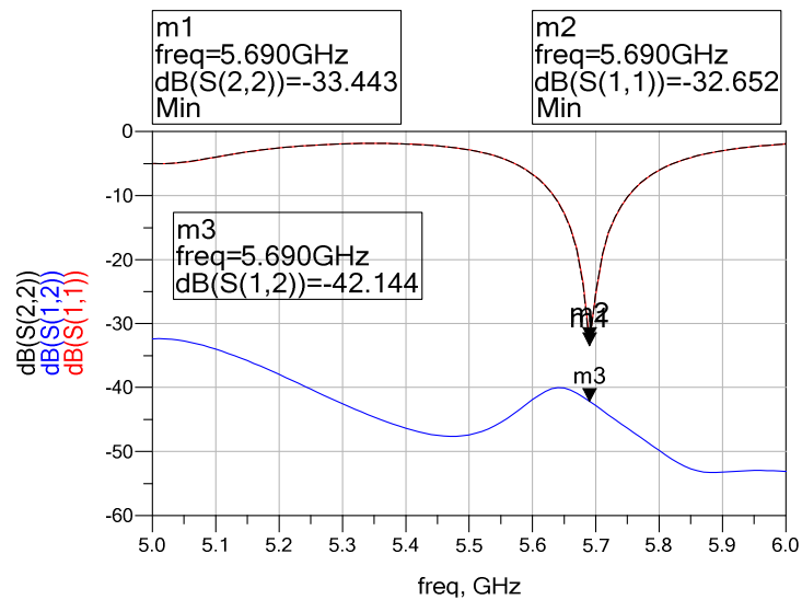
Figure 5.28: Simulated S-parameters of two H-plane pin loaded patch antennas with metallic wall barrier.
