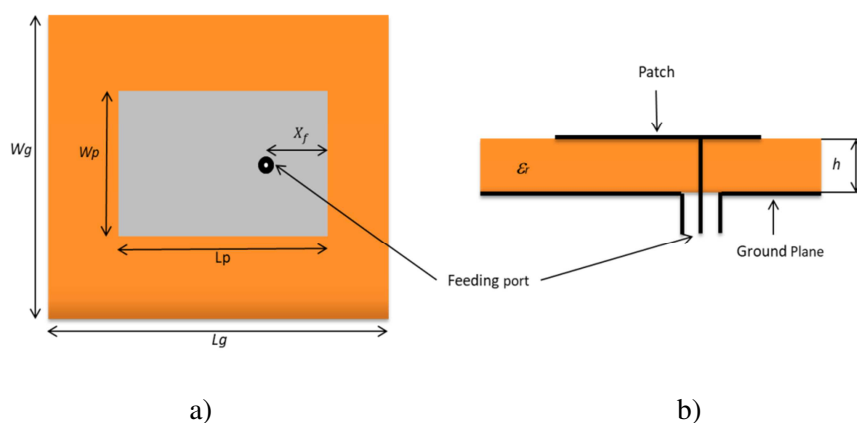
Figure 5.11: Conventional single patch antenna: a) top view, b) side view.
