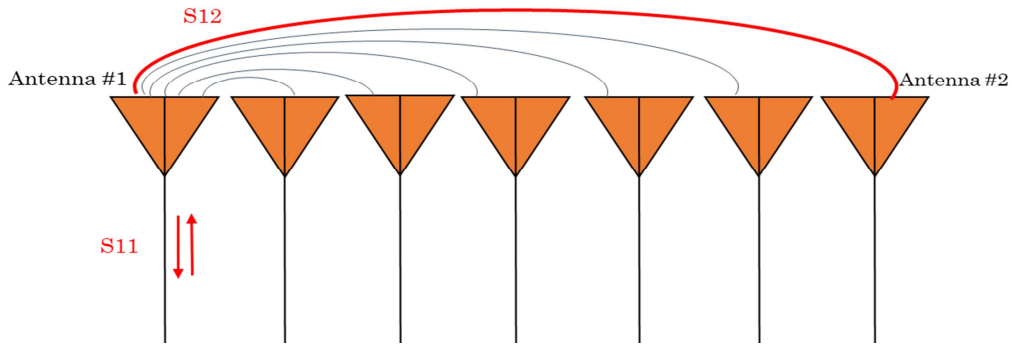
Figure 5.1: Mutual coupling phenomenon.
