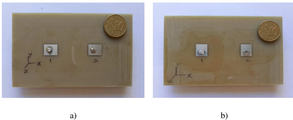
Figure 5.21: Two element conventional fabricated antenna array oriented along: a) E-plane, b) H-plane.
