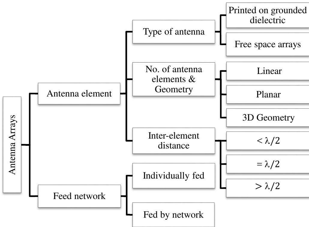
Figure 1.1: Antenna array selection flowchart according to a specified application.
