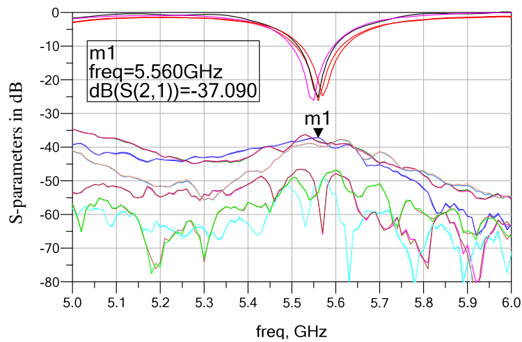
Figure 5.38: Measured S-parameters of pin loaded four patch antenna elements with metallic walls oriented along E-plane.
