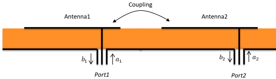
Figure 2.8: Individually fed two elements antenna system.
