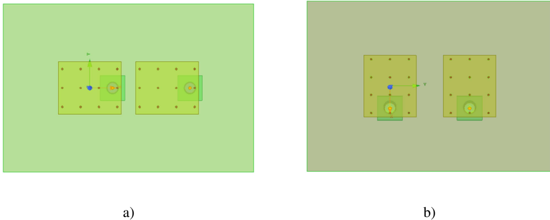
Figure 5.23: Pin loaded two element antenna array through 3D simulation: a) oriented along E-plane, b) oriented along H-plane.
