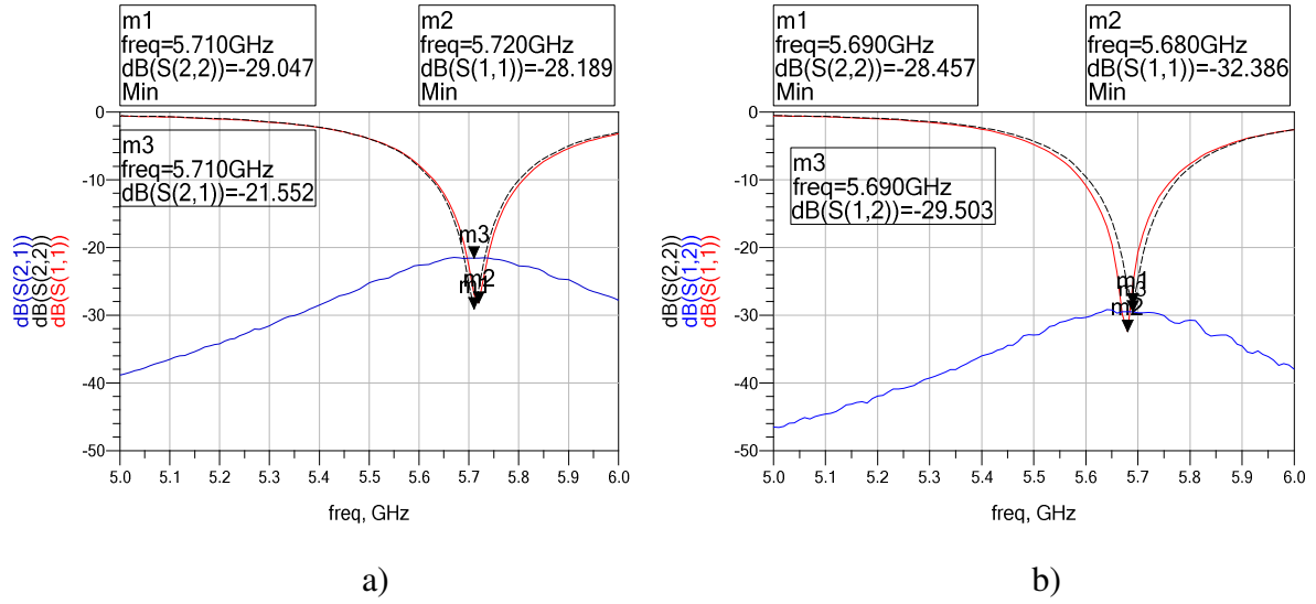
Figure 5.22: Measured S-parameters of two conventional antennas oriented along: a) E-plane, b) H-plane.
