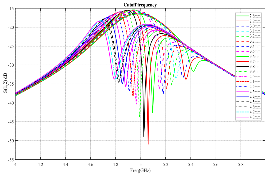
Figure 5.10: Parametric analysis of mutual coupling cutoff frequency shift with respect to the width ( W_1 ) of the DGS.
