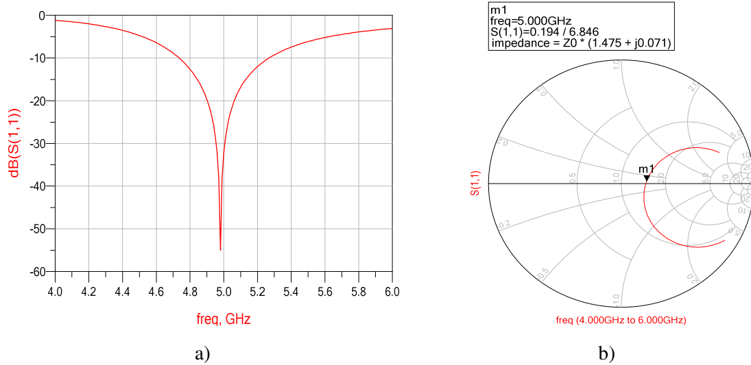
Figure 4.2: Single dipole antenna: a) optimized return loss, b) Smith chart.
