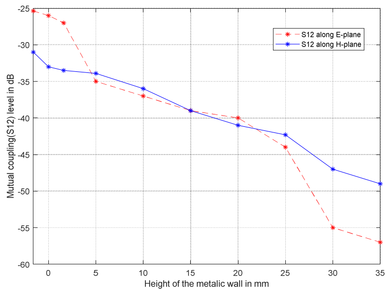
Figure 5.33: Parametric analysis of mutual coupling variation with respect to the wall height ( W_h ) in E and H-plane orientations in pin loaded patch antenna arrays.
