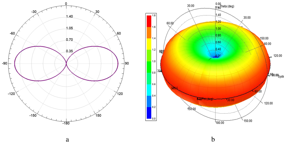
Figure 2.4: Radiation pattern of vertical dipole antenna in polar coordinates; a) 2D radiation pattern, b) 3D radiation pattern.
