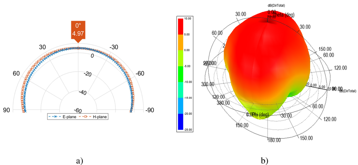
Figure 5.13: Simulated radiation pattern of conventional path antenna: a) 2D radiation pattern showing directivity in E and H-plane, b) directivity in 3D radiation pattern.
