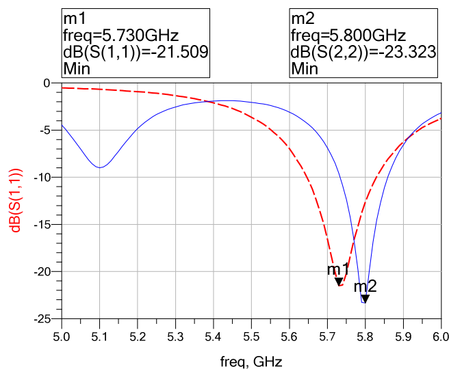
Figure 5.18: Return loss through measurement: Conventional patch antenna (dashed curve) and Pin loaded patch antenna (solid curve).
