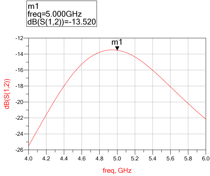
Figure 4.3: Mutual coupling test between two elements distanced half wavelength apart.
