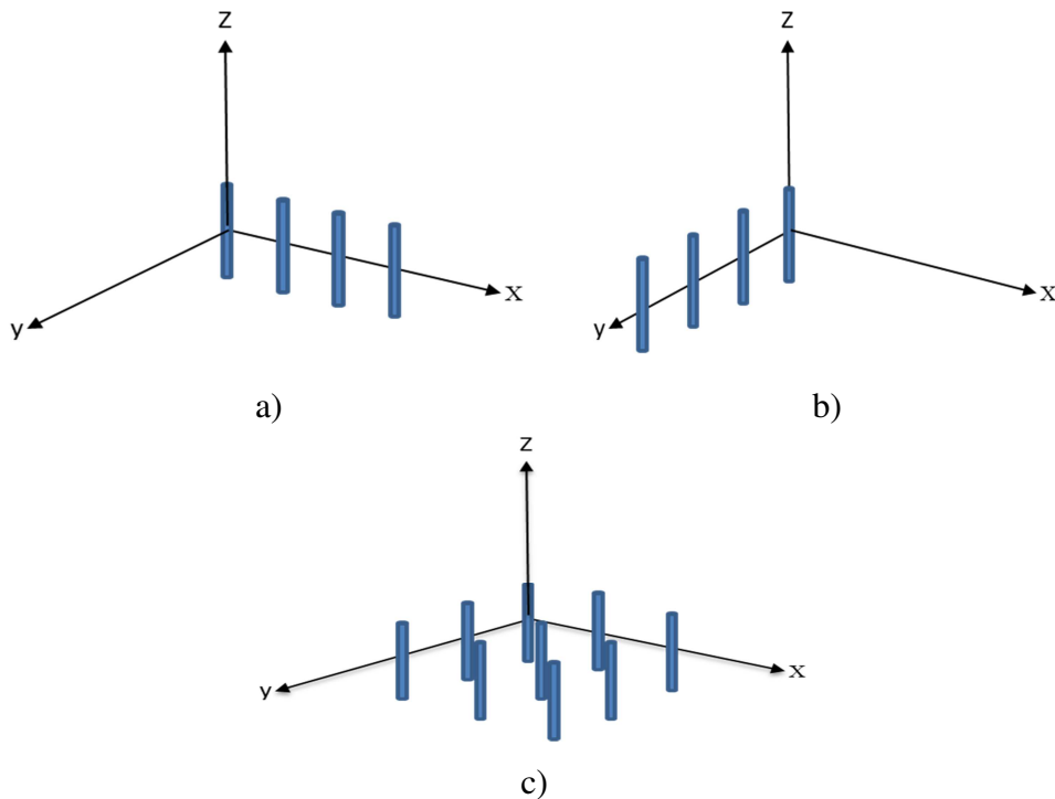
Figure 3.3: Short dipole antenna array combination arranged along; a) X-axis b) Y-axis c) XY-plane (Planar).
