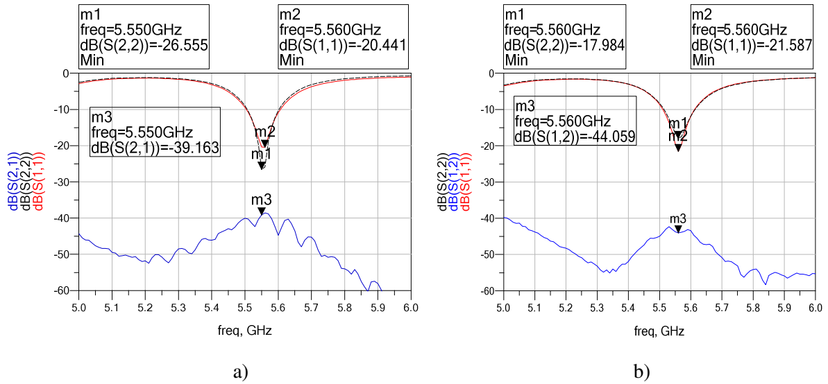
Figure 5.30: Measured S-parameters of pin loaded two antennas with metallic wall barrier through realization oriented along: a) E-plane, b) H-plane.
