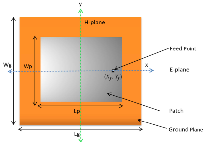
Figure 3.13: Patch antenna showing feed point, width and length and E and H-planes.
