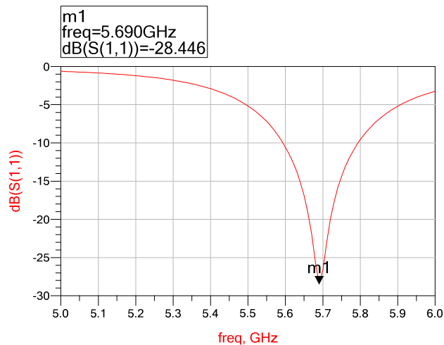
Figure 5.12: Simulated return loss of conventional patch antenna.
