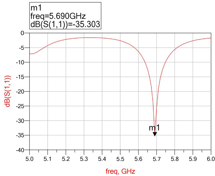
Figure 5.15: Simulated return loss of optimized pin loaded patch antenna.
