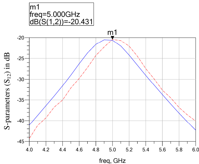
Figure 4.7: Mutual coupling between two E-plane antenna elements through: 3D simulation (solid curve), measurement (dashed curve).
