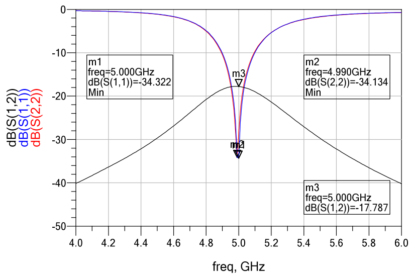
Figure 5.5: Simulated S-parameters without DGS.
