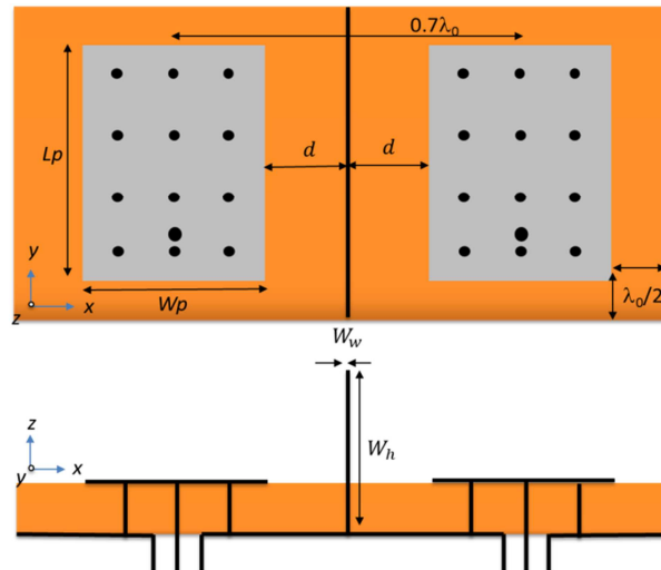
Figure 5.27: Two H-plane pin loaded patch antennas with metallic wall barrier.
