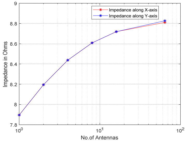
Figure 3.4: Input impedance variation of short dipole in array arranged along X-axis and Y-axis.
