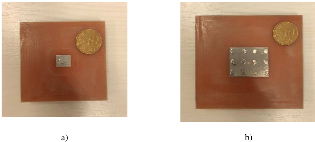
Figure 5.17: Laboratory prototypes: a) conventional patch antenna a) pin loaded patch antenna
