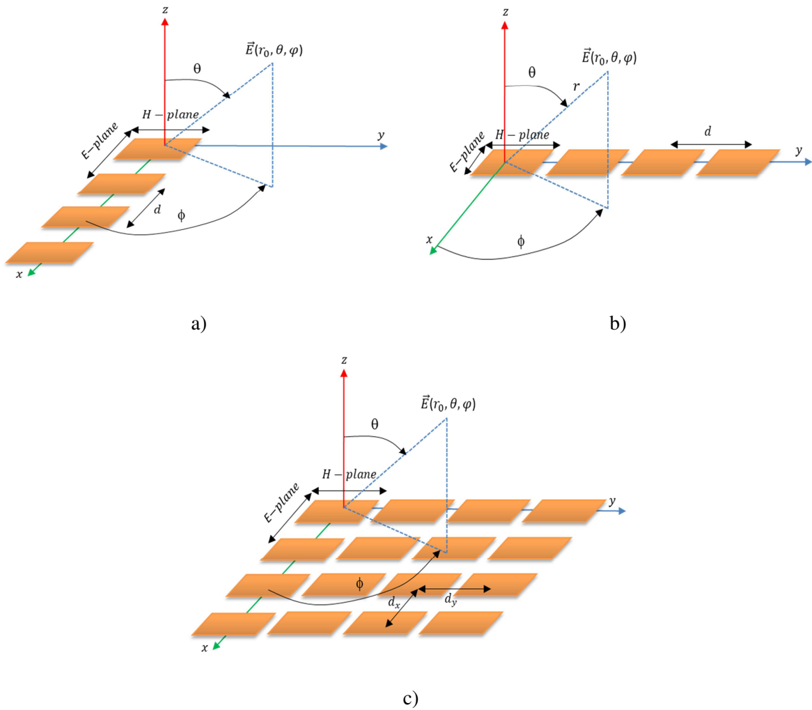
Figure 3.14: Patch antenna array arranged along: a) X-axis (E-plane), b) Y-axis (H-plane), c) XY-plane
