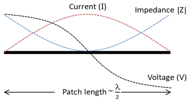
Figure 3.12: Current, voltage and impedance relation w.r.to patch antenna length[43].
