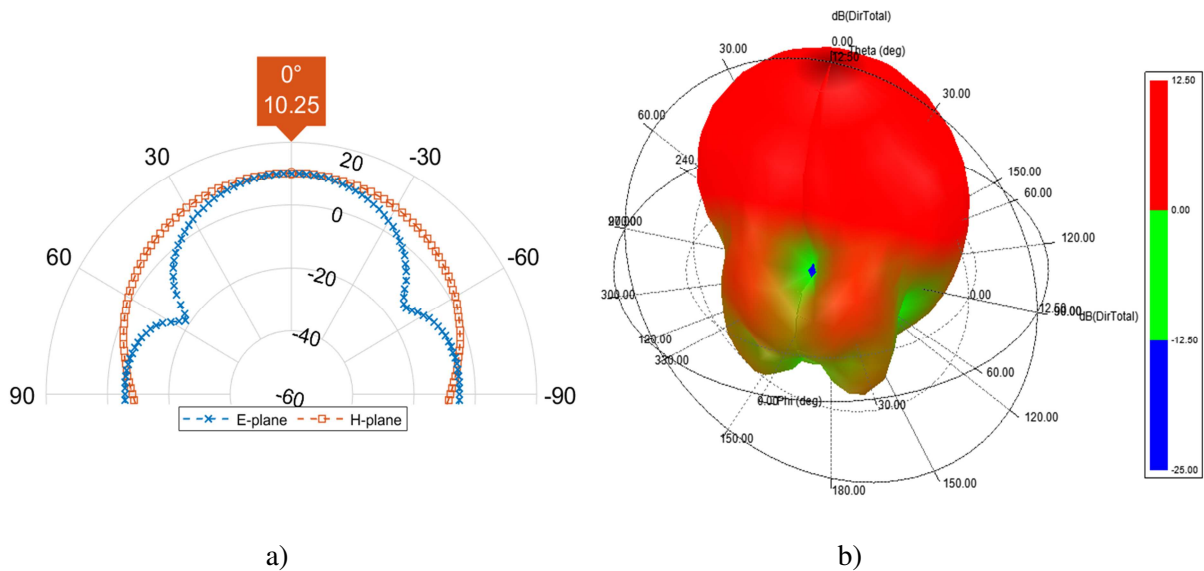
Figure 5.16: Simulated radiation pattern of pin loaded path antenna: a) 2D radiation pattern showing directivity in E and H-plane, b) directivity in 3D radiation pattern.
