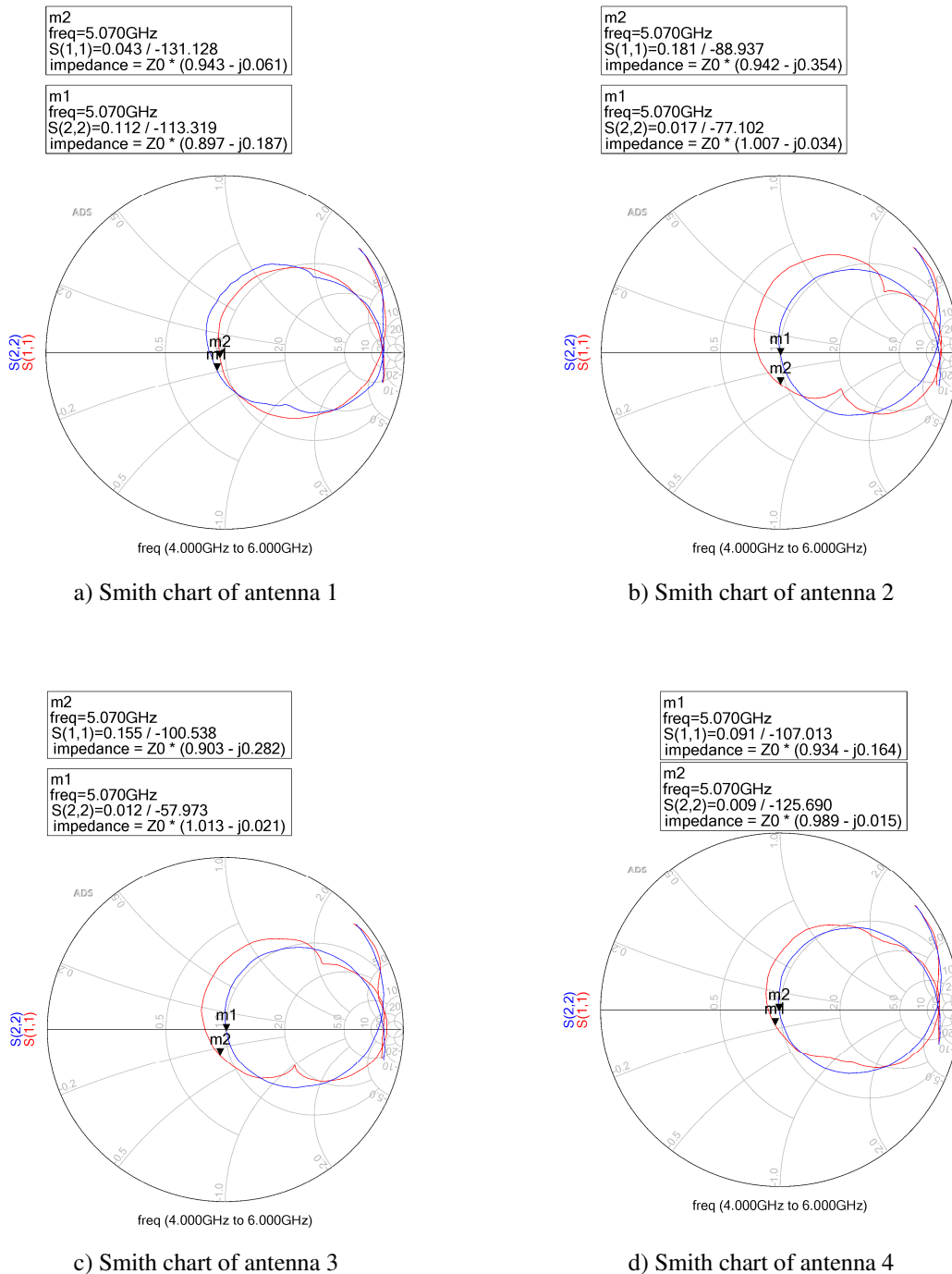
Figure 4.13: Smith chart of all four antennas; a) When one antenna is powered on (Red curve) and when all antennas are powered on(Blue curve), b) When one antenna is powered on (Blue curve) and when all antennas are powered on(Red curve), c) When one antenna is powered on (Blue curve) and when all antennas are powered on(Red curve), d) When one antenna is powered on (Blue curve) and when all antennas are powered on(Red curve).
