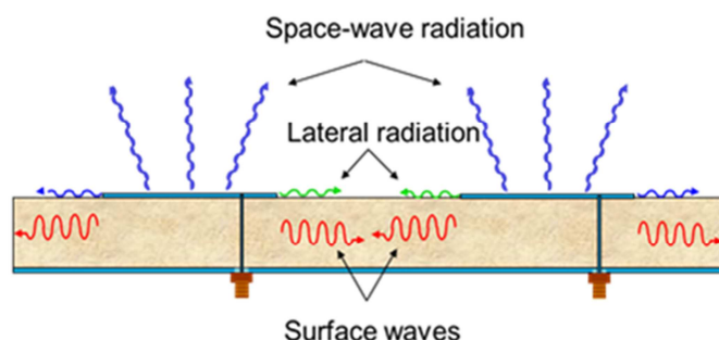
Figure 5.2: Mutual coupling mechanism in patch antennas.
