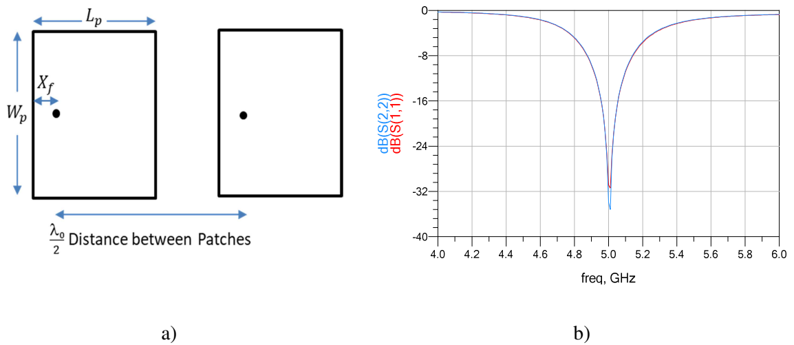
Figure 4.6: Simulated two patch antenna elements: a) arranged along E-plane, b) return loss.
