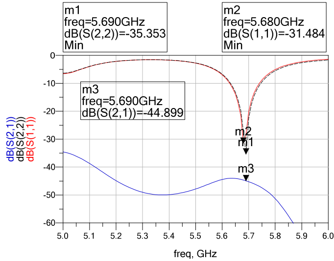
Figure 5.26: Simulated S-parameters of two E-plane pin loaded patch antennas with metallic wall barrier.
