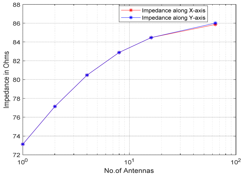
Figure 3.7: Input impedance variation of resonant wire antenna array arranged along X-axis and Y-axis.
