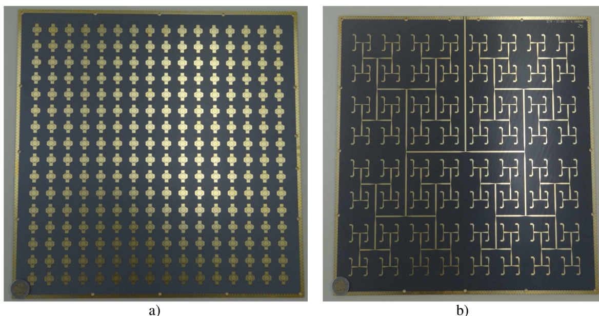
Figure 1.2: a) 16x16 Patch Antenna Prototype with front (Patch array) and b) back (feed network).
