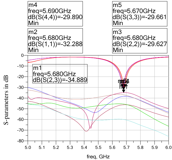
Figure 5.36: Simulated S-parameters of four pin loaded patch antenna elements with metallic walls oriented along E-plane.
