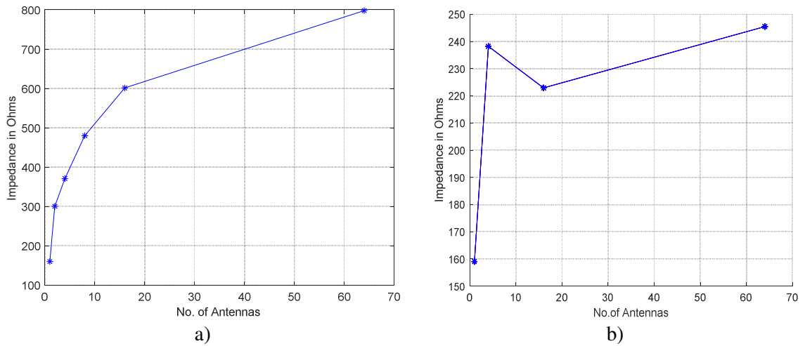
Figure 3.16: Input impedance variation due to total radiation versus number of antenna elements arranged along: a) H-plane, b) XY-plane.
