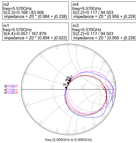
Figure 5.39: Smith chart of pin loaded four patch antenna elements with metallic walls oriented along E-plane.
