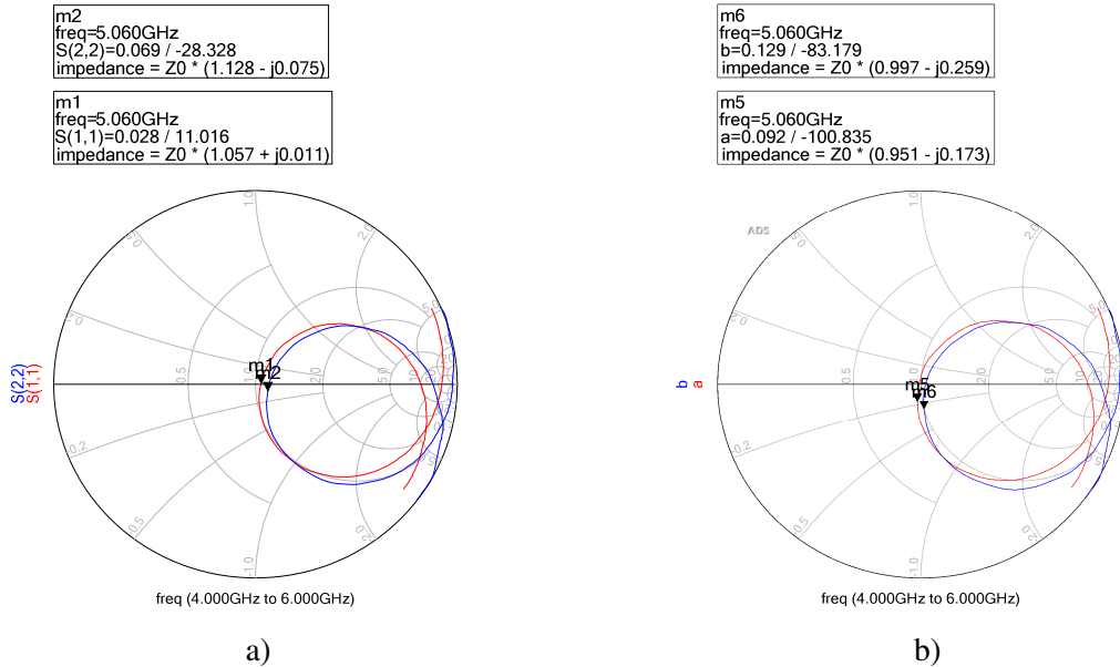
Figure 4.9: Smith chart of two antennas according to; a) Passive S-parameters, b) Active S-parameters according to equation 4.3.
