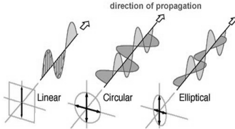
Figure 2.2: Electric field representation for linear, circular and elliptical polarization [27].
