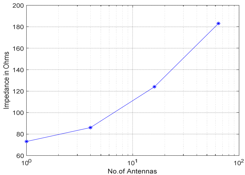
Figure 3.8: Input impedance variation of resonant wire antenna array arranged along XY-plane
