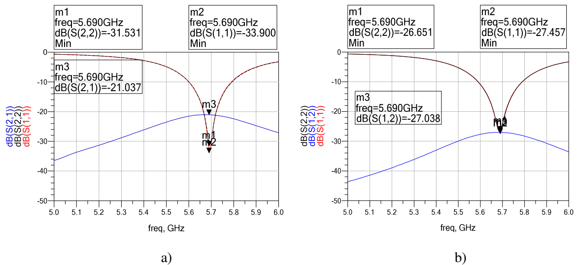
Figure 5.20: Simulated S-parameters of two conventional antennas oriented along: a) E-plane, b) H-plane.
