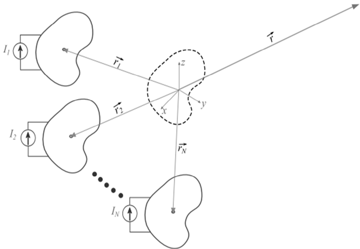
Figure 3.1: A schematic view of an antenna array.
