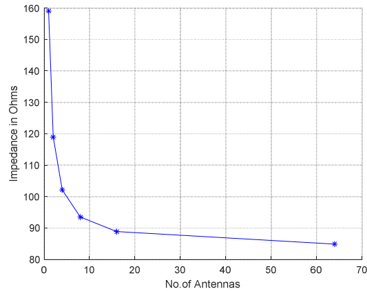
Figure 3.15: Input impedance variation due to total radiation versus number of antenna elements arranged along E-plane.
