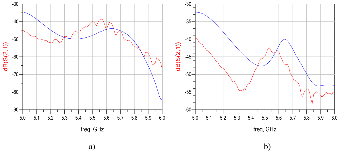
Figure 5.31: Mutual coupling through simulation (blue curve) and measurement (red curve): a) oriented along E-plane, b) oriented along H-plane.
