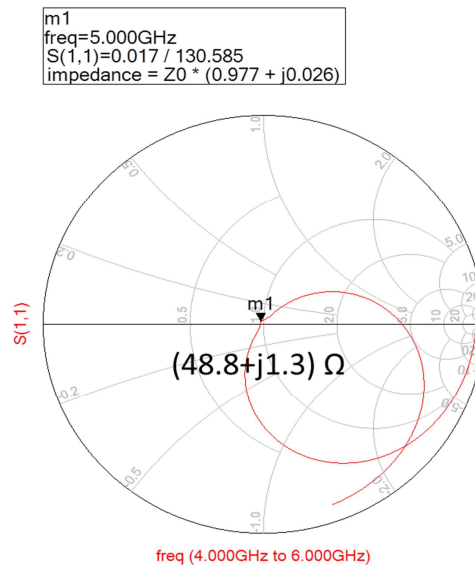
Figure 4.5: Smith chart of an optimized patch antenna.
