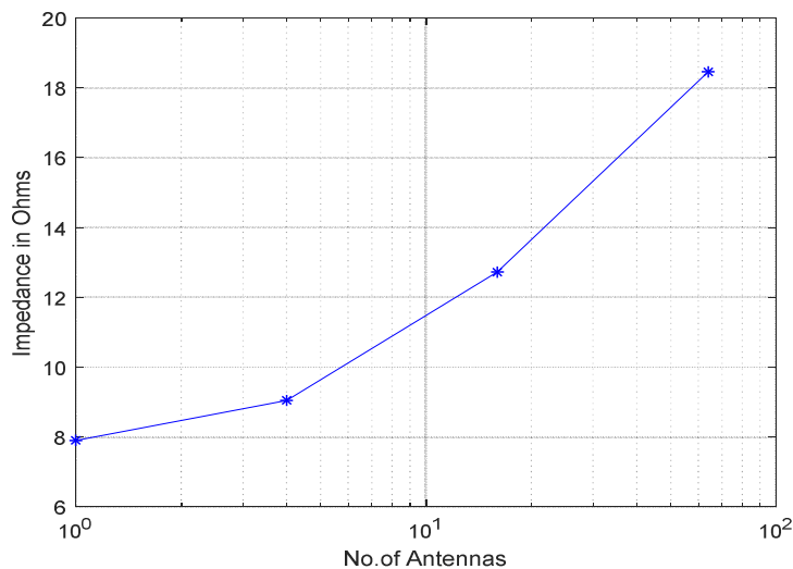
Figure 3.5: Input impedance variation of short dipole in array arranged along XY-plane
