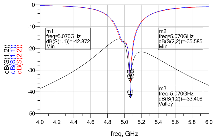
Figure 5.7: Simulated S-parameters with DGS.
