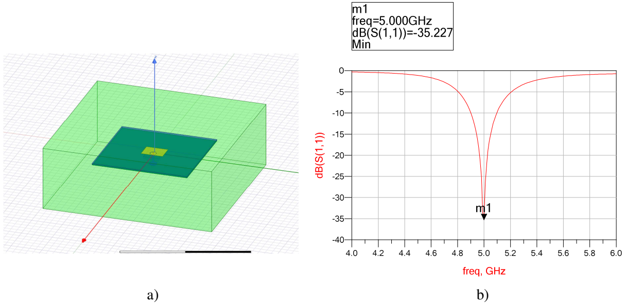
Figure 4.4: a) Simulated Patch antenna model in HFSS, b) return loss of the optimized patch.
