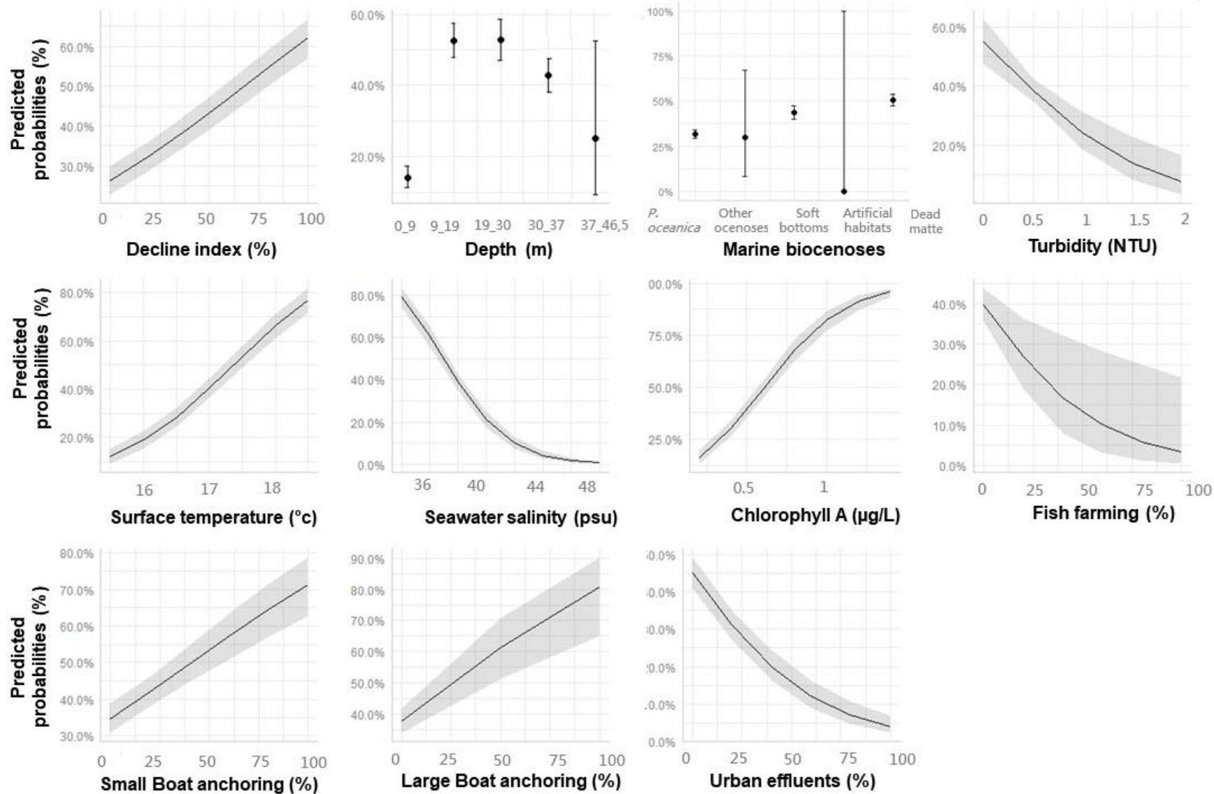
Figure 31 : Effect of each explanatory variable on the predicted probability of presence of both invasive alien macroalgae (IAM). The grey area represents the confidence interval. Note that to improve visualization, the Y axis scale is adapted to each variable. For human pressures, the X axis scale is given in scaled values (percentage of the maximum value, for the corresponding usable units)
