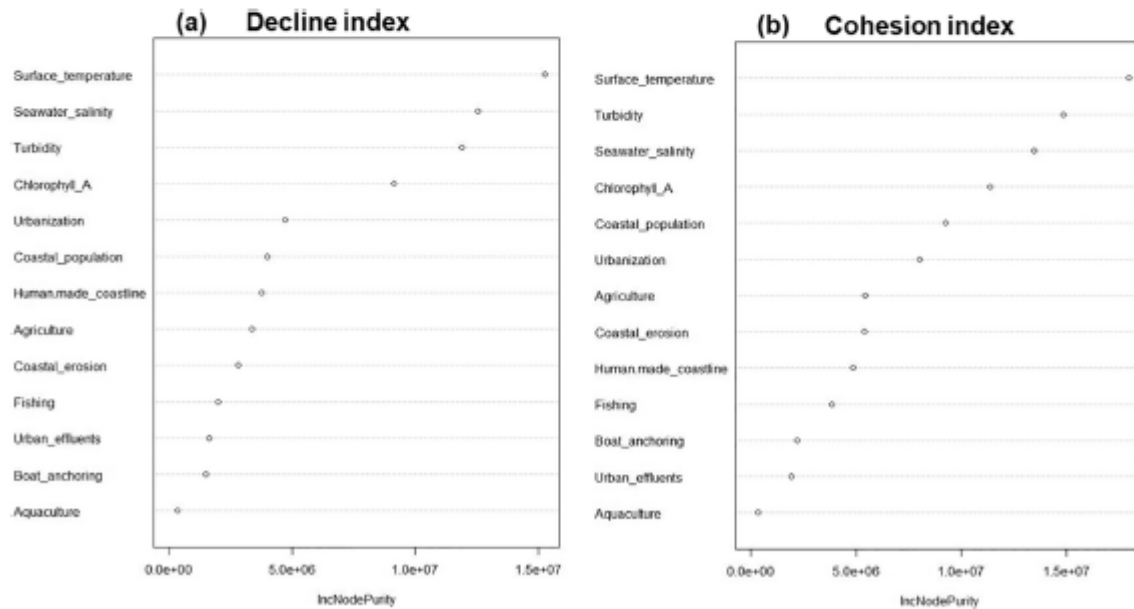
Fig. 2. Importance of each explaining variable relative to the seagrass decline index (a) and cohesion Index (b) with the Random Forest model respectively explaining 87% and 70% of the variance (grid cell size = 100 × 100 m).
