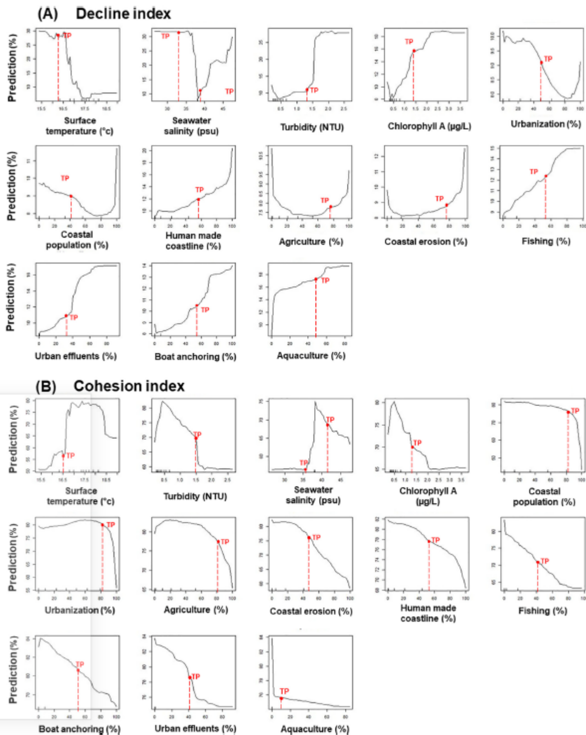
Fig. 3. Influence and response curves of each explaining variable on A) the decline index and B) the cohesion index of P. oceanica seagrass beds through the Random Forest model with 100 × 100m cells. Thresholds (TP) are indicated in red. Note that to improve visualization, the Y axis scale is adapted to each variable. The graphs are ordered according to the influence of the different factors on the indices (see Fig. 2). (For interpretation of the references to colour in this figure legend, the reader is referred to the web version of this article.)
