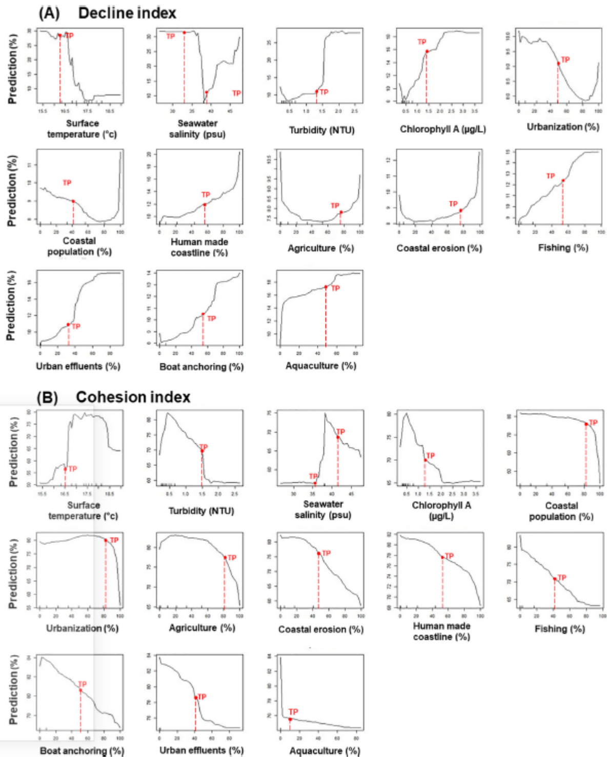
Fig. 3. Influence and response curves of each explaining variable on A) the decline index and B) the cohesion index of P. oceanica seagrass beds through the Random Forest model with 100 × 100m cells. Thresholds (TP) are indicated in red. Note that to improve visualization, the Y axis scale is adapted to each variable. The graphs are ordered according to the influence of the different factors on the indices (see Fig. 2). (For interpretation of the references to colour in this figure legend, the reader is referred to the web version of this article.)
