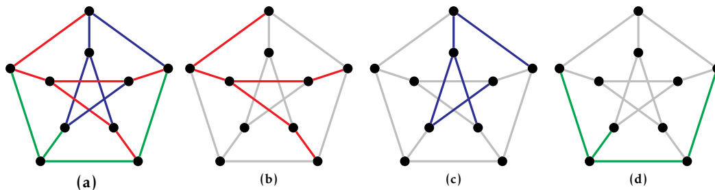
Figure 3.2: A decomposition (a) of the Petersen graph into three locally irregular subgraphs ((b) to (d)). Note that, in a resulting subgraph H of a locally irregular decomposition of a graph G , it is allowed to have d_H(u) = d_H(v) for an edge uv \in E(G) as long as uv \notin E(H) .
