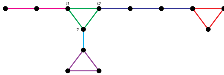
Figure 3.3: Iterative construction of a member of \mathcal{T} . The construction starts e.g. from the triangle uvwu with green edges. An even-length pending path with magenta edges is then attached to u . To v is then attached an odd-length path with cyan edges at the other end of which is attached a triangle with purple edges. To w is finally attached an odd-length path with blue edges at the other end of which is attached a triangle with red edges. Every graph obtained after some of these successive steps is also a member of \mathcal{T} .
