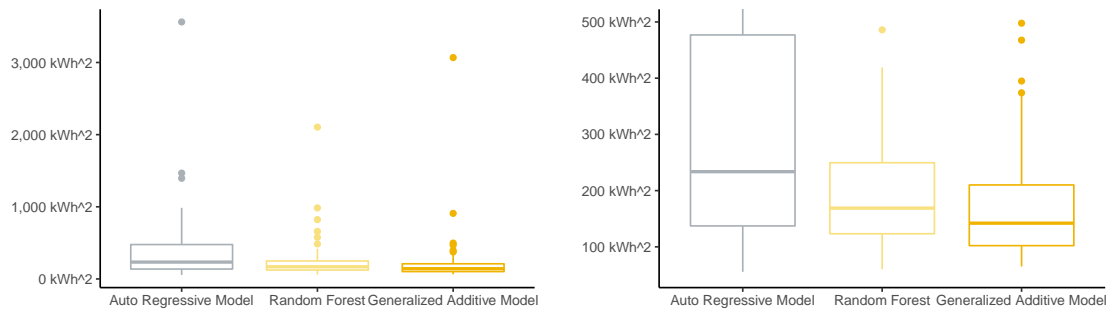
Figure 6.11 – Distribution over the test period of daily mean squared error of global consumption benchmark forecasts (auto-regressive model, generalized additive model, random forest). Left picture: original boxplots; Right picture: boxplots trimmed at 500 \text{ kWh}^2 .
