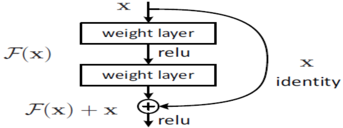
Figure 4.11 – An example of Skip connections [He et al., 2016].
