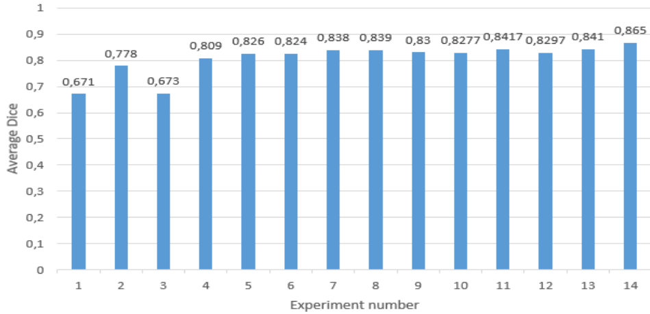
Figure 4.15 – The effect of class-weighting on the CNNs performance. Horizontal axis represents the experiment number in the table 4.3 (i.e., No.). The vertical axis represents the average Dice score of each experiment ( Table 4.3 column 10).
