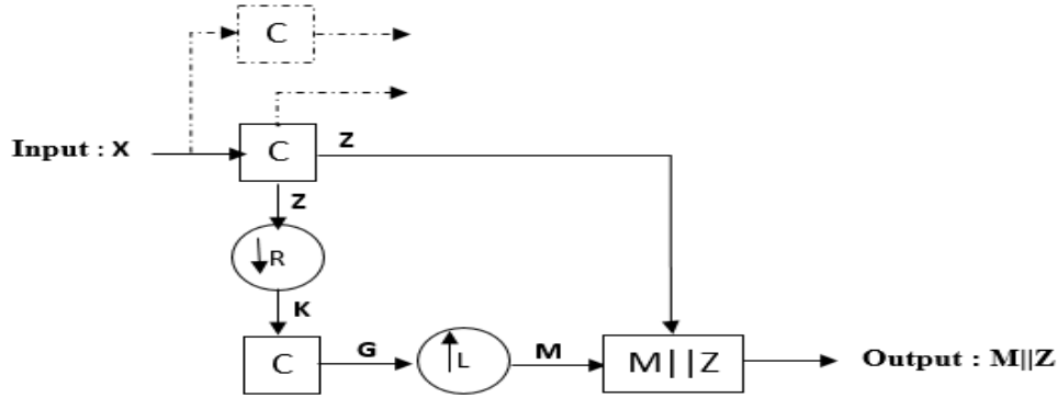
Figure 4.9 – An illustration of visual area V1. C is a convolution operator, Z and G are feature maps, K is the output of Pooling layer, M is a high-resolution feature map, \downarrow R is a pooling layer, \uparrow L is an upsampling operator, M || Z is a concatenation layer between M and Z. Also, the continuous lines are direct and skip connections, and dashed lines are used to build the second module of visual area V1 (i.e. DenseConnectionOCM).
