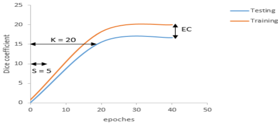
Figure 5.2 – Illustration of an example of the stopping criteria curve. EC is the Error's change, K is the total number of epochs, S is the number of iterations. The online class weighting algorithm stops after satisfying the following conditions: EC , K , S periods.
