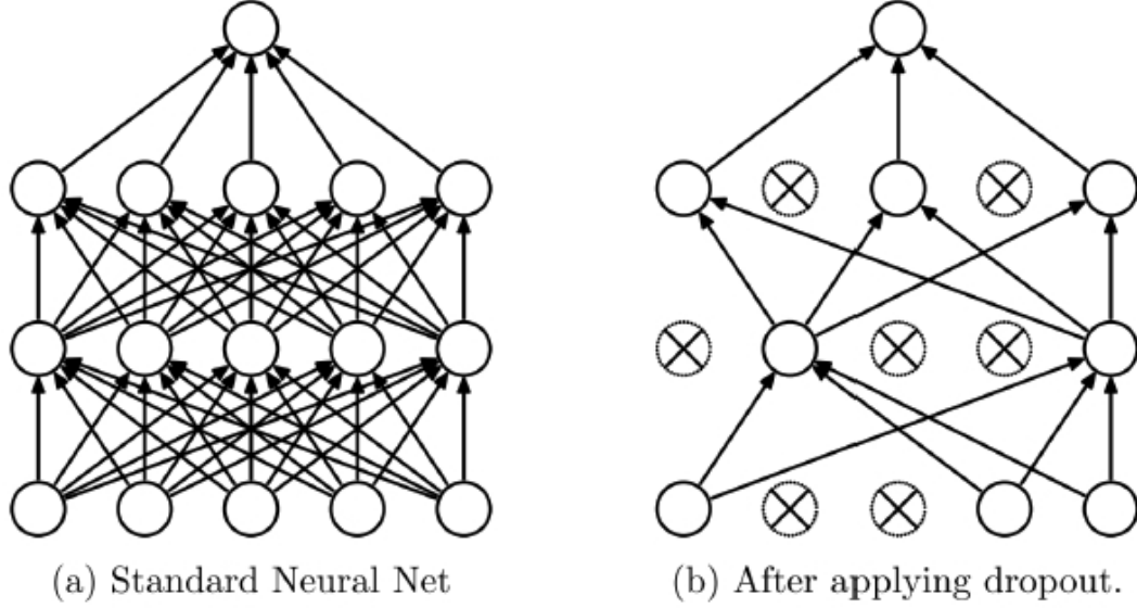
Figure 3.13 – Example of Dropout technique with different "dropout rates" for each layer. Left: is a fully-connected neural network. Right: is the same fully-connected neural network, where we randomly eliminate each hidden unit with a predefined probability. Figure from [Srivastava et al., 2014].
