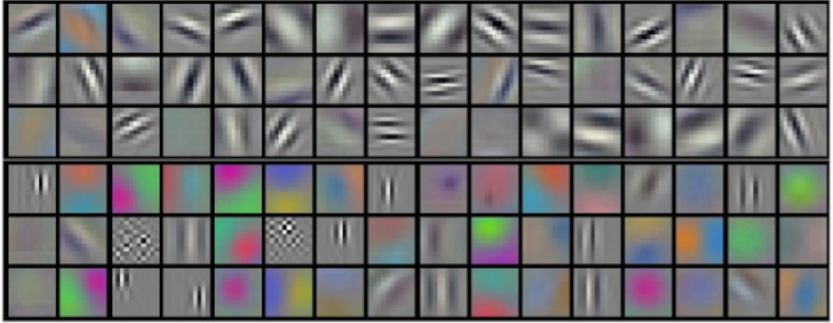
Figure 3.1 – Visualization of the first convolutional layer 's filters of the AlexNet model [Krizhevsky et al., 2012]. Those filters are trained to detect lower-features such as lines and edges in a different directions.
