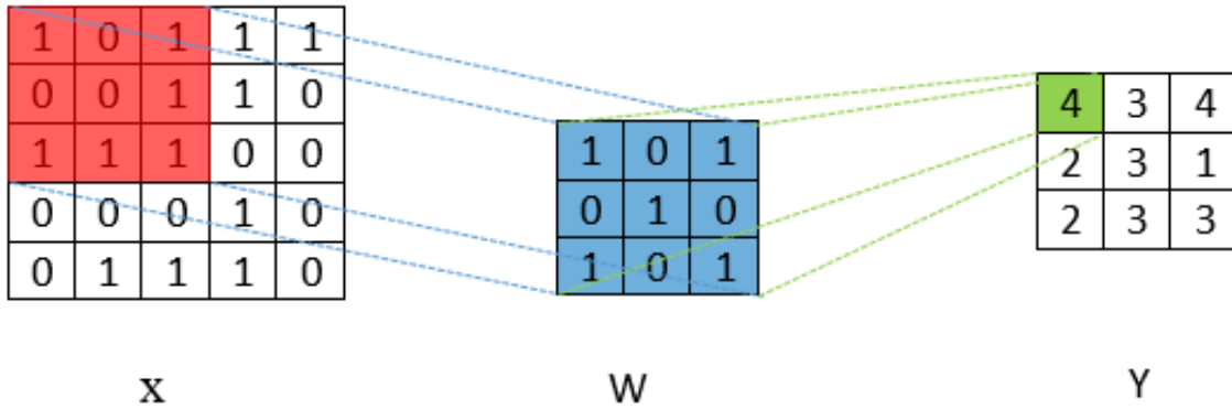
Figure 3.2 – An illustration of Convolution Operation on a single-channel image (Equation 3.2). Feature maps (Y) is the result of convolving the input (X) with a Filter (W).
