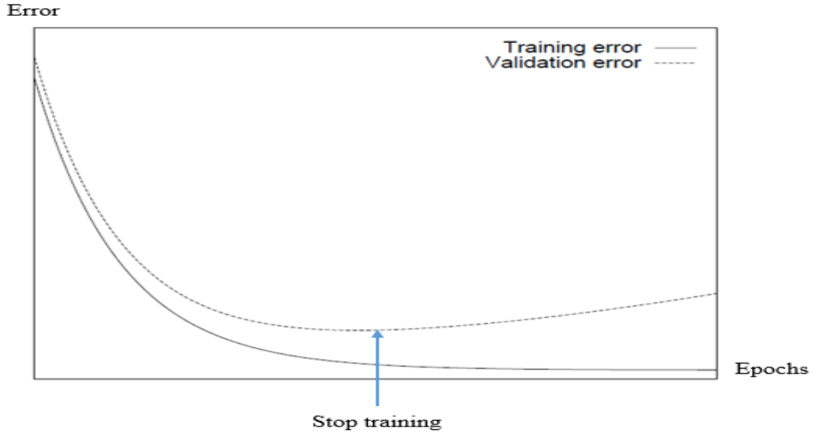
Figure 4.18 – An illustration of the early stopping technique. The figure shows the training and validation error curves. The principal axes are the epochs and the error value. Based on figure 1 [Prechelt, 1998]
