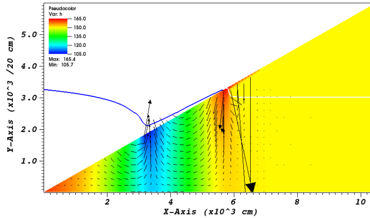
Figure 12.6: Snapshot of hydraulic head contours at t = 57.5 s for the end of the first backwash. Most velocities are less than 1 cm/h.
