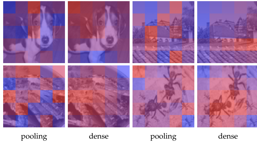
Figure 16.3: Examples overlaid with CAM [514] using ResNet-12 (cf. §16.7) trained with GAP or DC (16.6). Blue (red) is low (high) activation for ground truth. Top: Base classes ( walker hound , tile roof ). Bottom: Novel classes ( king crab , ant ).
