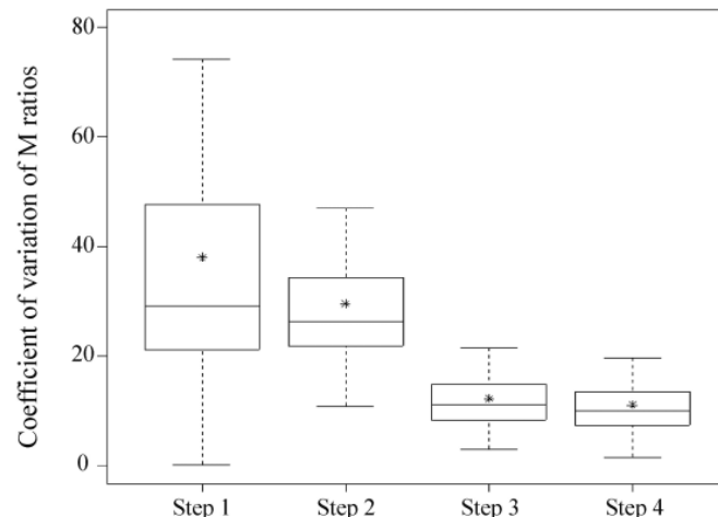
Figure 5. Decrease of the coefficients of variation of expression ratios, along the different MADSCAN analysis procedure steps. The expression values were from experiment 2, using 2 \times 2 replicate chips with four replicate spots for each gene. The 'box' in a 'box and whisker' plot shows the median of the values as a line, the mean as an asterisk and the first (25th percentile) and third quartile (75th percentile) of the expression values distribution as the lower and upper parts of the box, respectively. The 'whiskers' shown above and below the boxes represent the largest and smallest observed values, respectively, that are less than 1.5 box lengths (interquartile range) from the end of the box. When the box is in the middle of the whiskers, the data are probably more evenly distributed (steps 3 and 4). Steps 1 to 4 are as in Figure 1.
