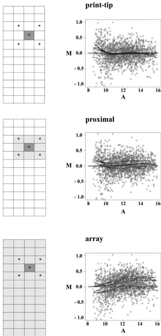
Figure 4. Comparisons between global, proximal and local normalization procedures. Five individual lowest fitness curves corresponding to five arbitrarily chosen blocks (asterisks) are represented according to each of the three spatial normalization modes. Light gray blocks represent an example of blocks chosen for selection of invariant genes, to normalize the raw M -values in the dark gray block, in each of the three modes. Invariant genes within the dark gray block are part of the invariant population used in each mode. The superposition of the five selected curves shows how uncontrolled local variations may influence the final expression values. The expression values presented here were from experiment 2.
