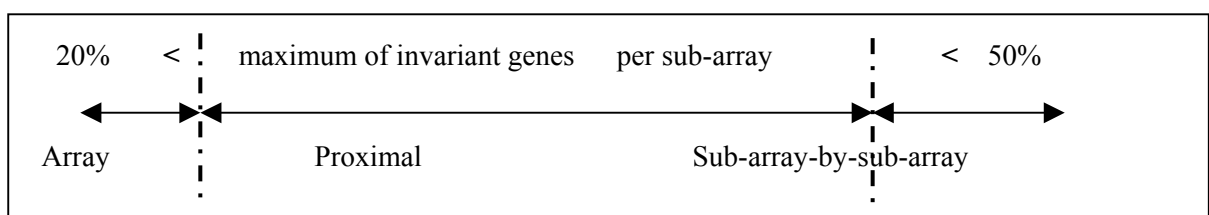
Figure 53. Interval of application for the different spatial approaches of normalization.
