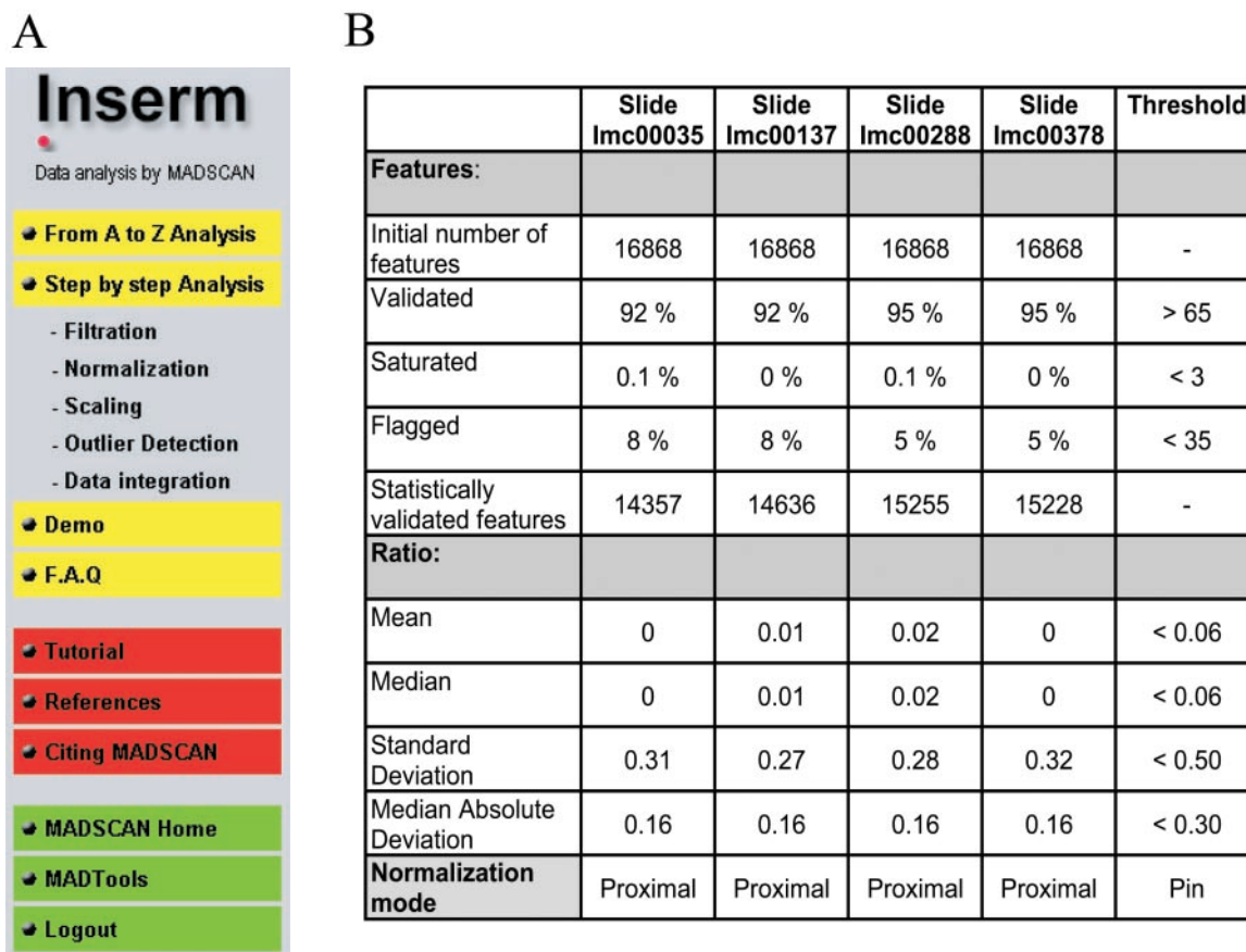
Figure 8. Web-accessible starting menu (A) and data summary page (B) in the MADSCAN module. For details, see pp. 22 and 27 in the tutorial. Note the definition of threshold values concerning the quality of the chip(s) and related expression measurements.
