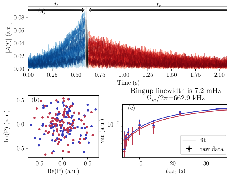
Figure VII.10: (a) For the parameters t_{\text{wait}} = 0.1\text{s} , t_b = 0.7\text{ s} and t_r = 4.5\text{ s} , a few experimental time traces are presented, taken from the BM2 sample. From those traces the waveform is inferred using the method proposed in [MFL13]. In blue (red) are presented the part of the time trace that is used to produce the blue (red) dots of (b) and (c). (b) complex representation of the scalar products of each trace with the inferred waveform. (c) Variance of the scalar products for different value of t_{\text{wait}} , together with an exponential fit. The inferred linewidth is \sim 7\text{ mHz}
