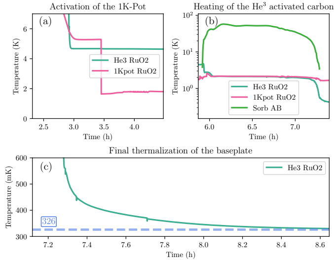
Figure III.12: Evolution of the different temperatures in the last cooling steps. (a) Activation of the 1K-pot. (b) Manual heating of the \text{He}^3 activated carbon. (c) Condensation of the \text{He}^3 leading to the baseplate temperature of \sim 326 mK.
