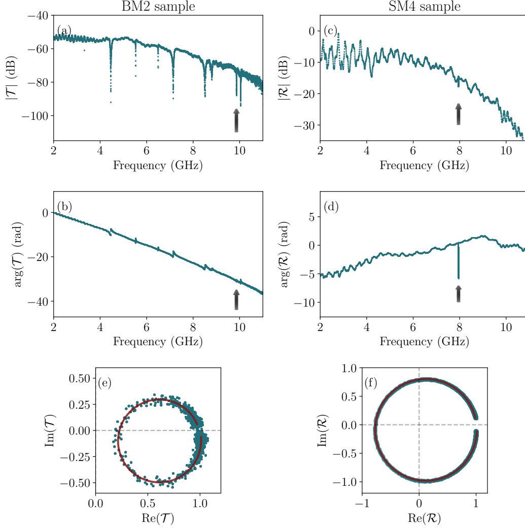
Figure IV.9: Comparizon of the large VNA scans, showing the amplitude (top) and angle (bottom) of the reflection (after design optimization, on the right) or transmission (before design optimization, on the left) of the sample. The angular drift is due to a delay corresponding to the time a signal needs to travel through he whole transmission lines. The resonance frequency is each time indicated with a black arrow. (e) Smith chart of the data close to the resonance for a resonator before design optimization. Data are represented by blue dots and a fit is represented in red. The extracted parameters are \omega_c/2\pi \approx 9.86 GHz, \eta \approx 0.79 , \kappa/2\pi \approx 792 kHz, and \kappa_0/2\pi \approx 166 kHz. (f) Smith chart of the data close to the resonance of a resonator after design optimization. Data are represented by blue dots and a fit is represented in red. The extracted parameters are \omega_c/2\pi \approx 7.95 GHz, \eta \approx 0.89 , \kappa/2\pi \approx 1.36 MHz, and \kappa_0/2\pi \approx 150 kHz.
