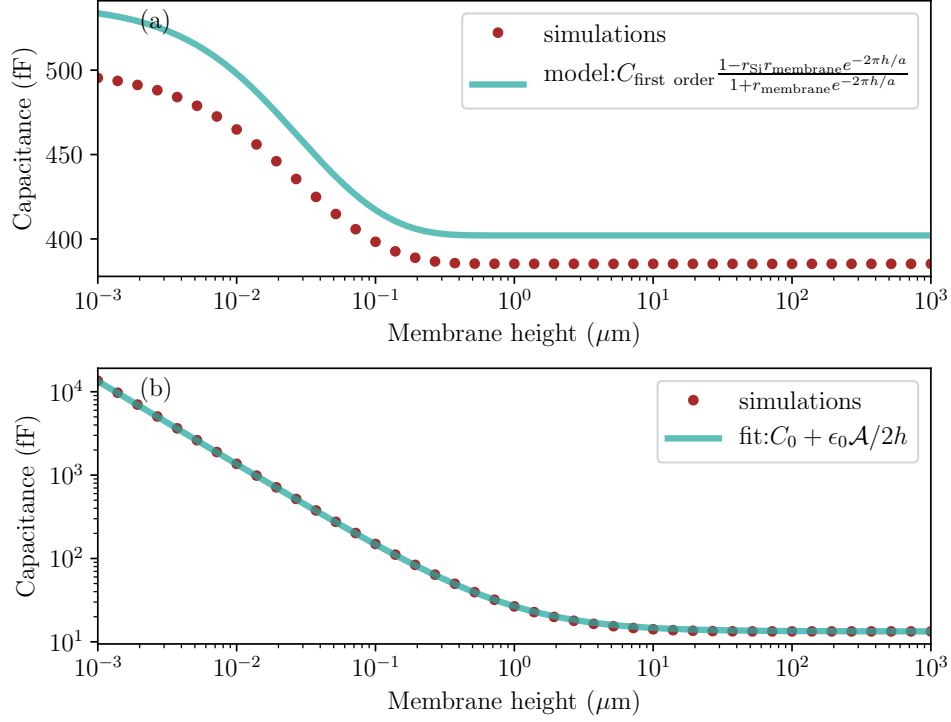
Figure III.5: Comparison between numerical simulations and approximate analytical formulas: (a) (dots) DC simulations using the software Sonnet of an interdigitated capacitance with a teeth period 2a = 1 \mu\text{m} , teeth length p = 80 \mu\text{m} , and 44 teeth per electrode (see sketch in (c)). The membrane thickness is 100 nm. (line) Model using formula III.1.32. There are no free parameters. (b) (dots) simulations of a mechanically compliant capacitor with two squared electrodes of width 55 \mu\text{m} separated by a distance of 20 \mu\text{m} (see sketch in (d)). (line) Model using the formula III.1.33. The only free parameter is the parasitic capacitance C_0 , which is set to be equal to the capacitance at the largest membrane height.
