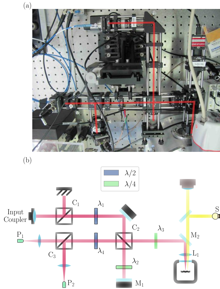
Figure II.5: (a) Interferometer picture. The light path is colored in red. (b) Schematics describing the optical elements
