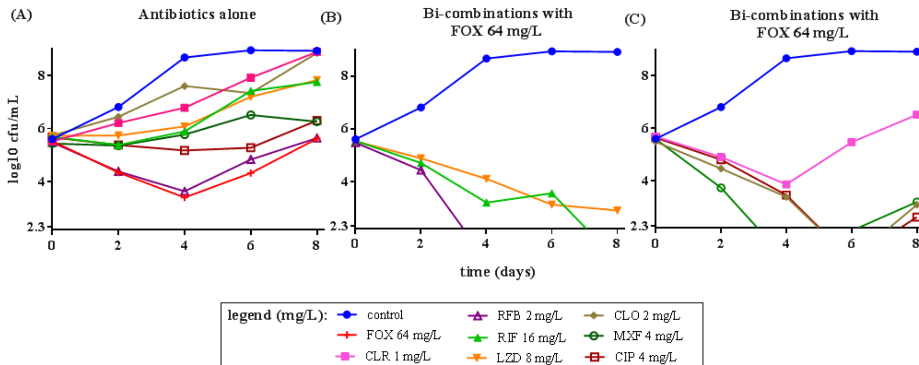
Figure 3: Effect of various combinations on M. abscessus T28. (A) Activity of several screened antibiotics alone, (B) cefoxitin in combination with linezolid, rifampicin and rifabutin, and (C) cefoxitin in combination with clarithromycin, clofazimine, moxifloxacin and ciprofloxacin. 50% amount of FOX was compensated each 24h up to 8 days to maintain the FOX amount constant throughout the experiment. CFUs were determined at the interval of 2 days. The dashed line represents the limit of quantification.
