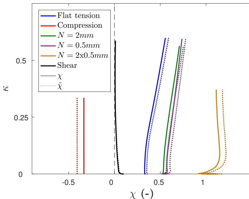
Figure 3.30: Loading paths for the different geometries. \dot{\epsilon} \simeq 10^{-3}\ \text{s}^{-1} , T = 25\ ^\circ\text{C} and Transverse direction TD. From left to right: simple compression, tension-induced shear, flat tension, simple notched ( R = 2\ \text{mm} and R = 0.5\ \text{mm} ) and double notched specimens. Definitions for the stress triaxiality can be found in Equations 1.1 and 3.38.
