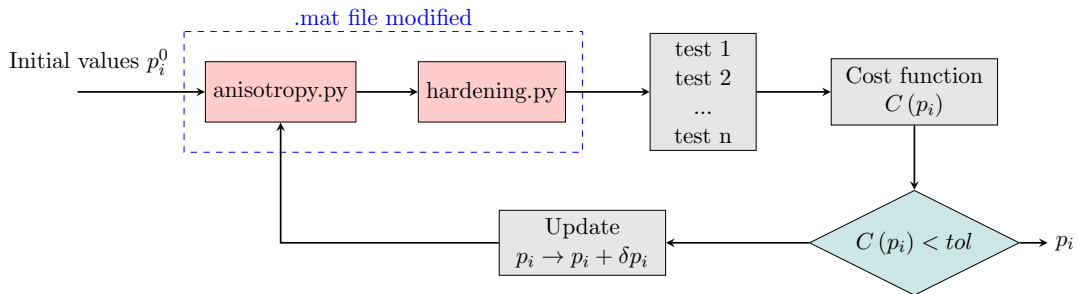
Figure 2.7: Inverse identification flowchart.
