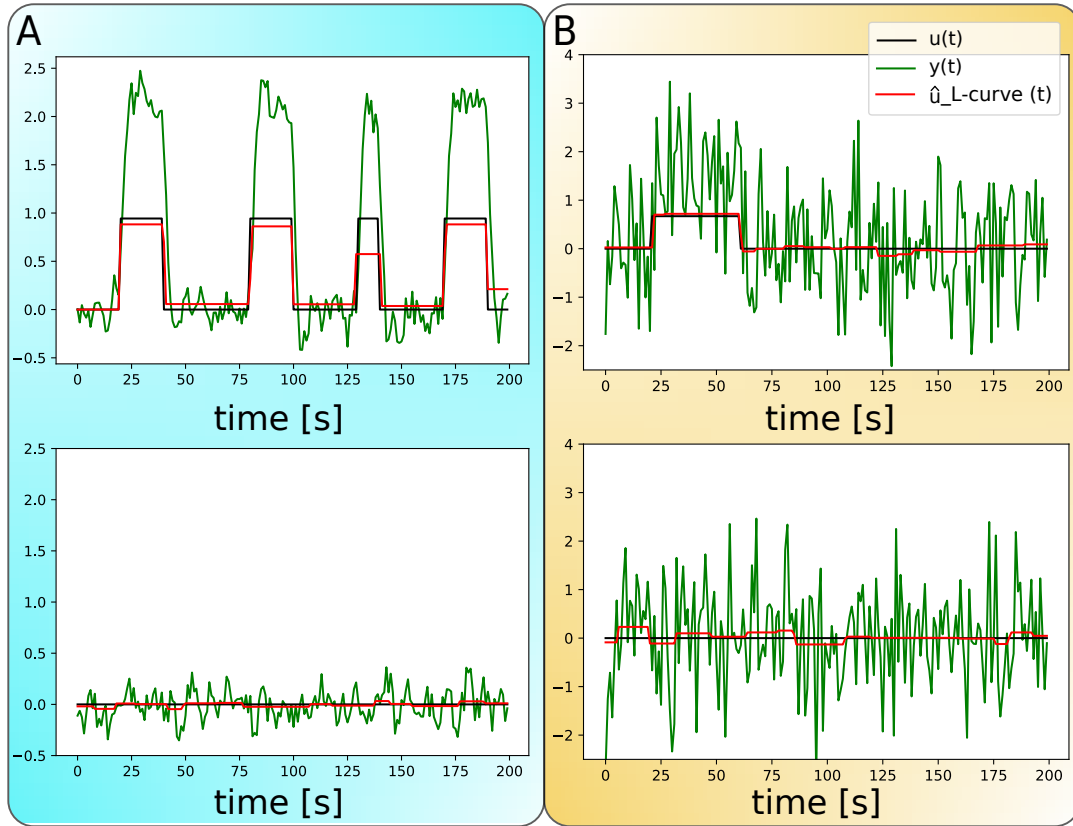
FIGURE 3.12: Reconstructed activity-inducing signal \hat{u}(t) obtained with our approach (red) superimposed on the ground truth u(t) (black) and simulated fMRI signal y(t) (green). The plots in the blue square are taken from exemplificative voxels and are related to activation A with pSNR = 5.17 dB; the ones in the yellow square are related to activation B with SNR = 5.12 dB. Vertically, for both A and B, the plots show that our approach is able to discern between an activation and a non-activation.
