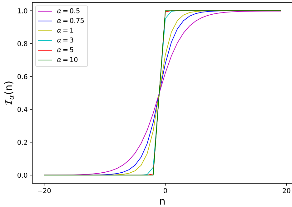
FIGURE A.5: The plot shows for different values of \alpha the function I_\alpha(n) defined in Eq. (A.13), normalized by the factor S defined in Eq. (A.35). The graphs show that for greater values of \alpha , the filter is sharper, whereas if \alpha is smaller, the filter has a smoother shape.
