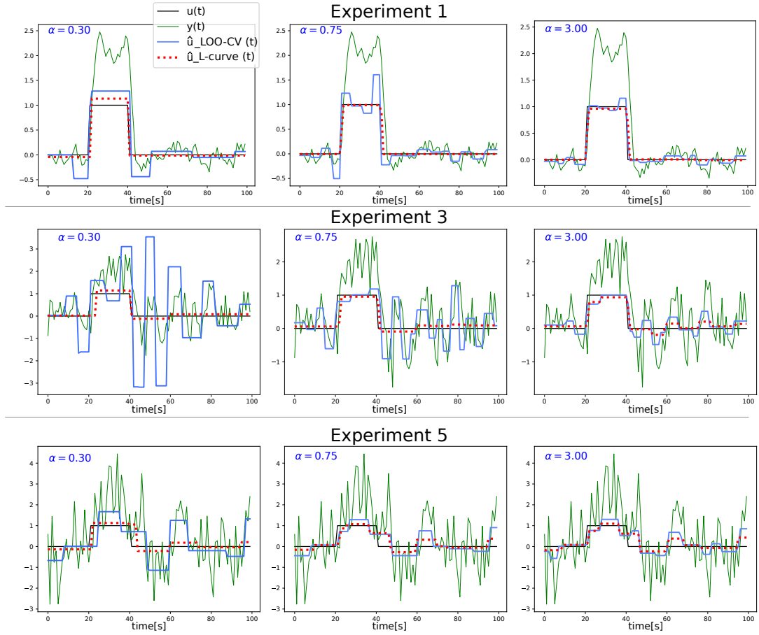
FIGURE 3.8: The graphs in the plots show examples of the recovered activation using the mixed Least Angle Regression (LARS)-L-curve approach (in red) and the mixed LARS and leave-one-out cross-validation (LOO-CV) (in light blue) superimposed on the ground truth activation in black and the noisy synthetic fMRI time series (in green). Each row shows a different experiment, meaning different noises applied to the ground truth activation and each column refers to a specific \alpha used in the \alpha -filter. In experiments 1, 3 and 5 the added noise was coming from different sources: block-type noise ( \epsilon_b ) to simulate false-activations, model noise \epsilon_m and additive noise \epsilon_a . The standard deviations of \epsilon_m and \epsilon_a increases from experiment 1 to 5. The plots show that the recovered activations using the L-curve-based approach are much closer to the ground truth compared with LOO-CV. The L-curve-based approach shows results that are closer to the ground truth in terms of amplitude for bigger alphas. For \alpha = 0.75, 3 , results are similar, while in contrast with those given by \alpha = 0.3 .
