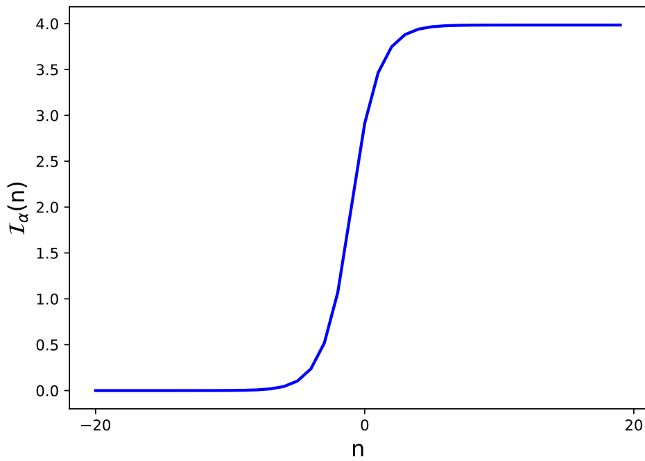
FIGURE A.3: Function I_\alpha(n) defined in Eq. (A.13), for S = -1 and \alpha = 1 .
