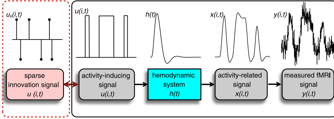
FIGURE 2.2: fMRI signal model. From left, u_s(i, t) is the spike train (innovation signal) which induces the activation for each voxel i . u_s(i, t) is the derivative of u(i, t) which represents the activation and it is assumed to be a block-type signal. h(t) is the hemodynamic response function, that convolved with the activity-inducing signal u(i, t) gives the activity-related signal x(i, t) . y(i, t) represents the measured fMRI signals for each voxel i , which is obtained by adding noise to the activity-related signal. (Figure adapted from Karahanoğlu et al. [6]).
