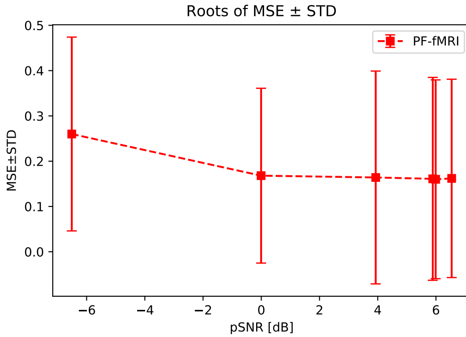
FIGURE 4.8: The graph shows, for different peak-SNRs (pSNR), the roots of the mean square errors (MSEs) and standard deviation (STD) between the ground truth signal u(t) and the recovered signals \hat{u}_{PF-fMRI}(t) averaged across the voxels belonging to the gray matter.
