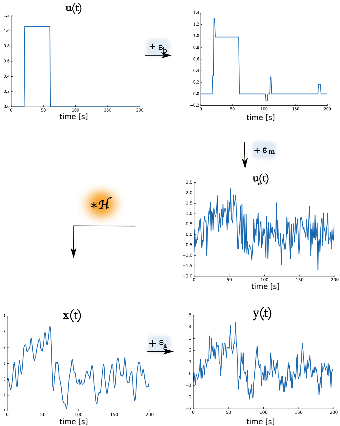
FIGURE 3.5: fMRI signal simulation. u(t) is the activity-inducing signal, a block of constant activation represented with a piece-wise constant signal. \epsilon_b is the block type noise and \epsilon_m the model noise which were consecutively added to the activity-inducing signal u(t) thus leading to u_n(t) before the convolution with the hemodynamic response function \mathcal{H} . x(t) is the activity-related signal, \epsilon_a is the additive gaussian noise and y(t) is the simulated acquired fMRI time course.
