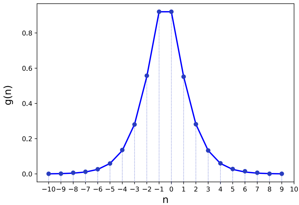
FIGURE A.4: Function g(n) defined in Eq. (A.15), for S = -1 and \alpha = 1 . The plot shows that \sum_{n=-\infty}^{-1} g(n) is equal to \sum_{n=0}^{+\infty} g(n) . This means that, if we compute \sum_{n=-\infty}^{+\infty} g(n) = \sum_{n=-\infty}^{-1} g(n) + \sum_{n=0}^{+\infty} g(n) this is equivalent to \sum_{n=-\infty}^{+\infty} g(n) = 2 \sum_{n=0}^{+\infty} g(n).
