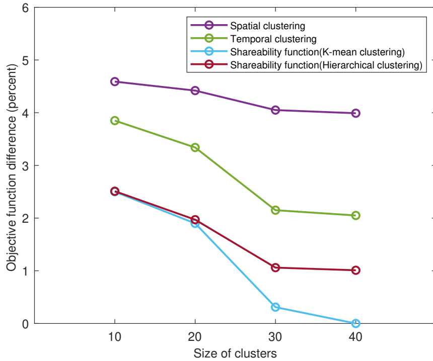
Figure 5.15: Comparing clustering methods' objective function (market-share=50%)
