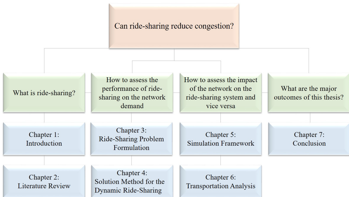
Figure 7.1: Thesis summary
