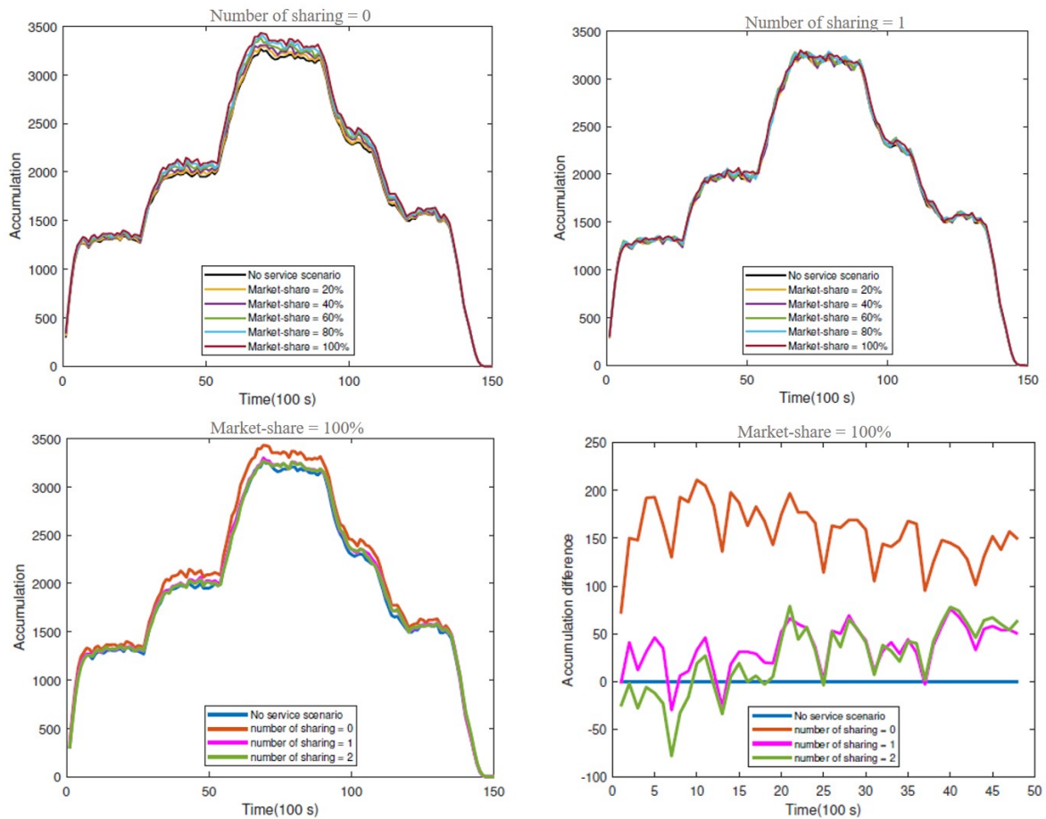
Figure 7.2: Medium-scale results
