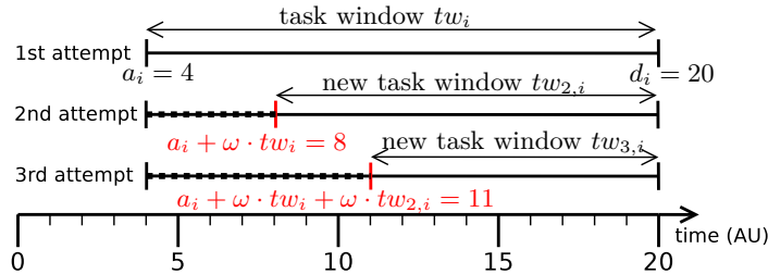
Figure 3.13 – Three scheduling attempts at \omega = 25\%
