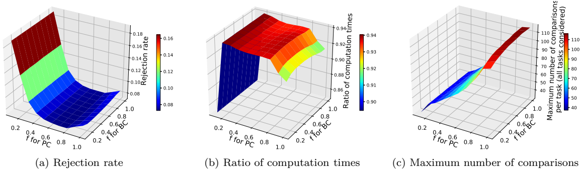
Figure 3.24 – Method of restricted scheduling windows as a function of the fractions of task window for the primary and backup copies (PB approach + BC deallocation, FFSS SbS; P = 14 ; TPL = 1.0 )
