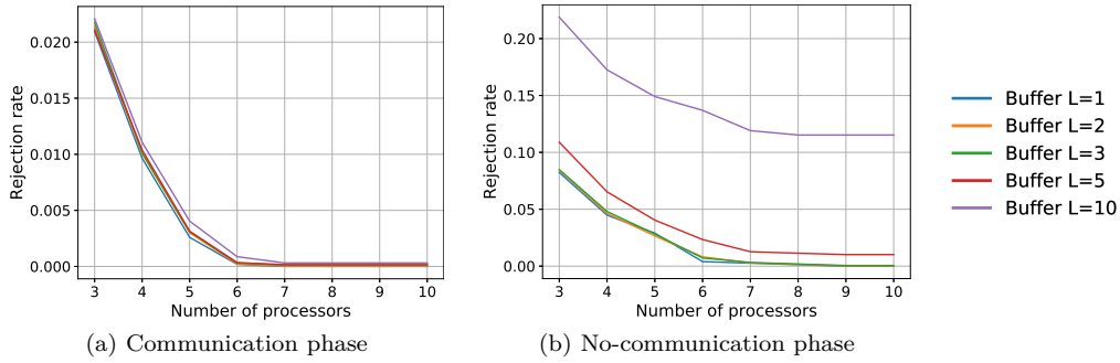
Figure 5.16 – Rejection rate as a function of the number of processors (ONEOFF; Scenario APSS)
