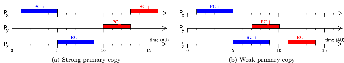
Figure 2.10 – Difference between strong and weak primary copies
