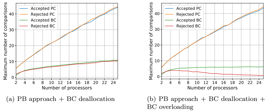
Figure 3.8 – Maximum number of comparisons per task as a function of the number of processors (FFSS SbS, TPL = 1.0 , no limitation on the number of comparisons)
