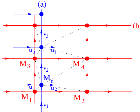
Figure 6.1: Interpolation of the pressure.
