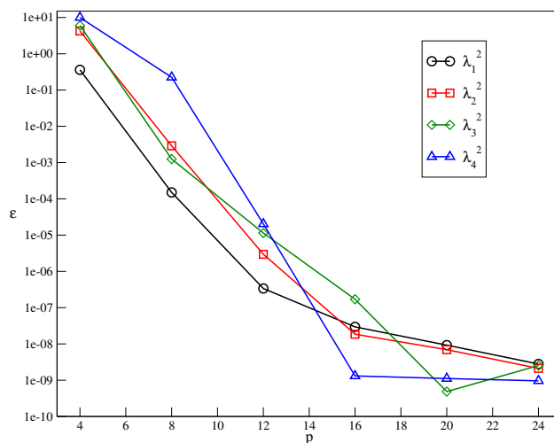
Figure 3.6: Convergence plots obtained using the divergence-free Galerkin explicit approach method for the four lowest divergence-free modes as a function of p .
