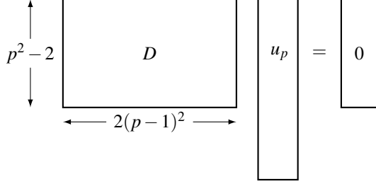
Figure 3.1: Algebraic system.
