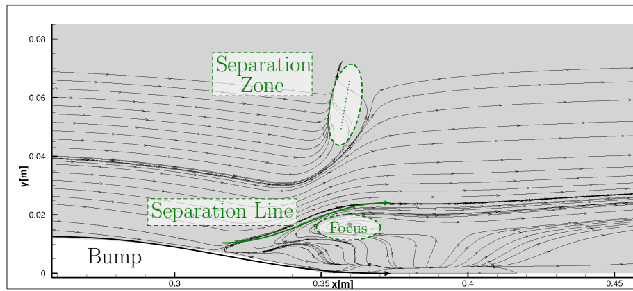
(b) RANS.
