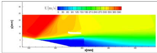
(g) U: z = 0 mm.
