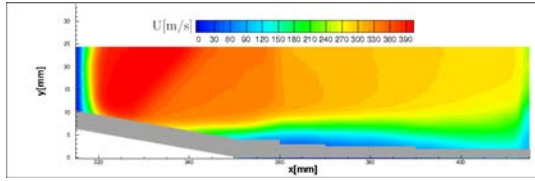
(c) U: z = -14 mm.
