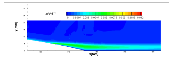
(j) u'v' : z = -14 mm.
