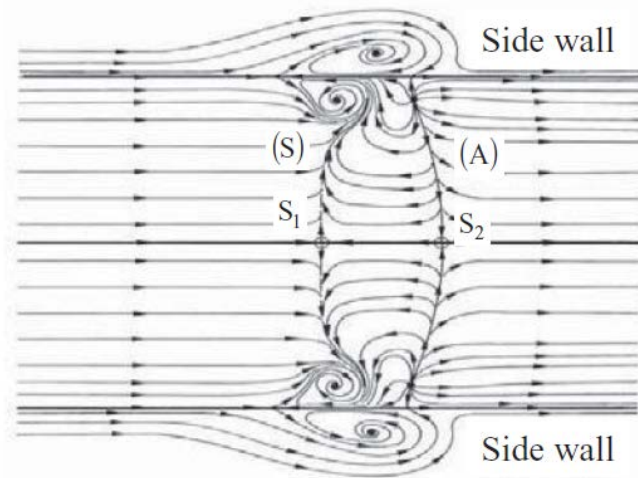
Figure I.19: 3D topology of friction lines of a SWBLI with separation in a channel flow from Babinsky and Harvey [6].
