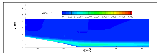
(l) u'v' : z = -26 mm.
