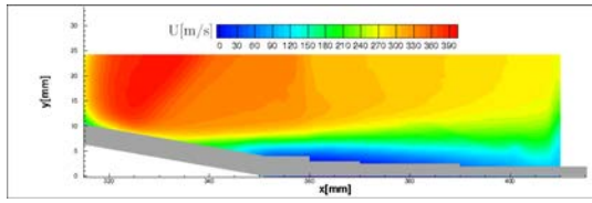
(a) U: z = 0 mm.
