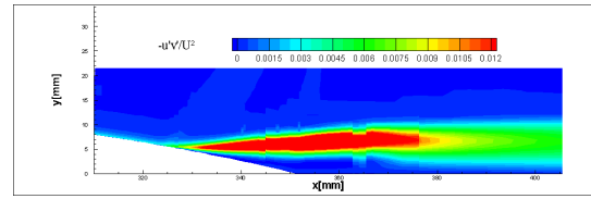
(h) u'v' : z = 0 mm.
