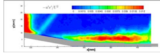
(b) u'v' : z = 0 mm.
