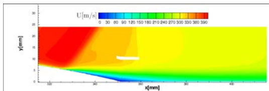
(i) U: z = -14 mm.
