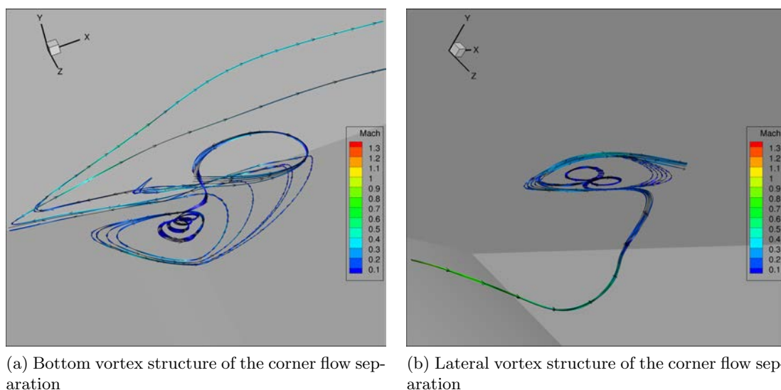
Figure III.10: Streamlines decomposition of the corner flow separation.
