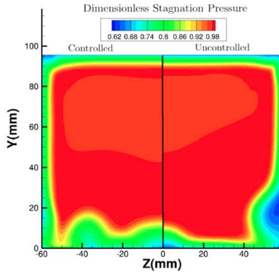
Figure IV.21: Non dimensionalized stagnation pressure on the transverse DC50 plane of the best controlled case of the second optimization-left- and uncontrolled case-right-.
