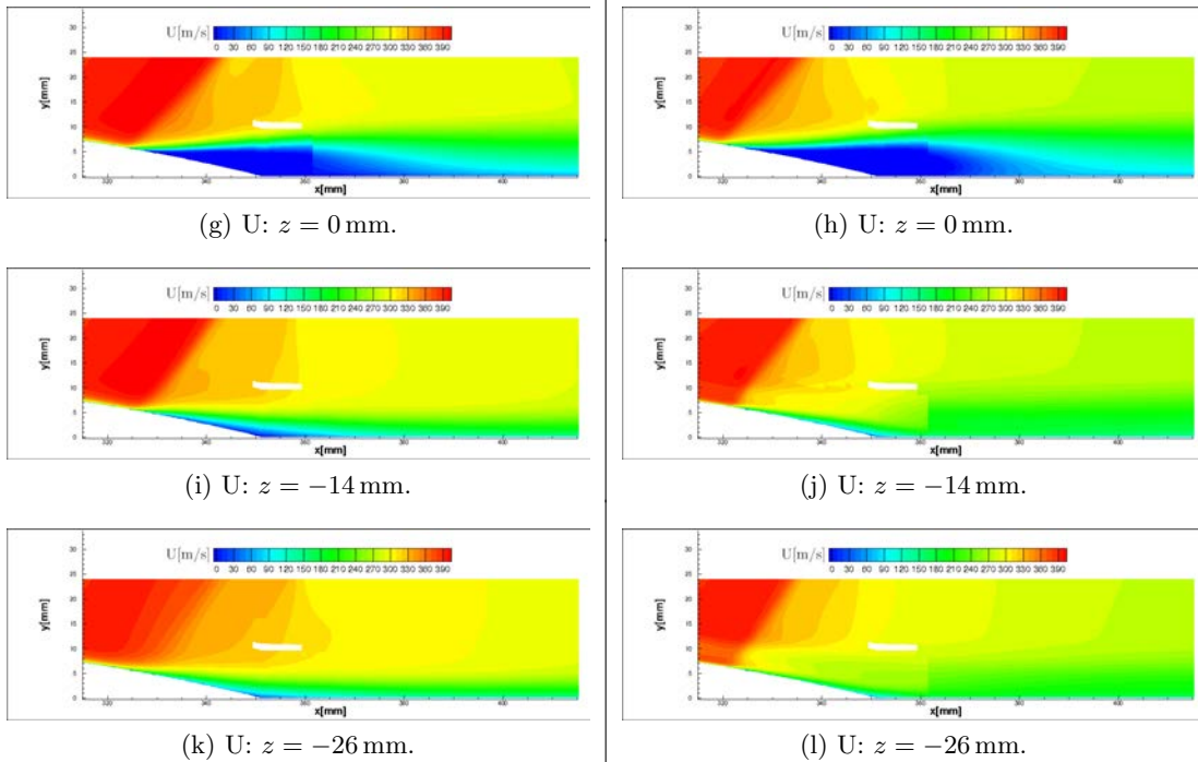
Figure VII.9: Comparison of longitudinal velocity fields given by the tomographic PIV and RANS modeling (respectively up and down) for the reference and Control 1 cases (respectively left and right), at three different lateral planes.
