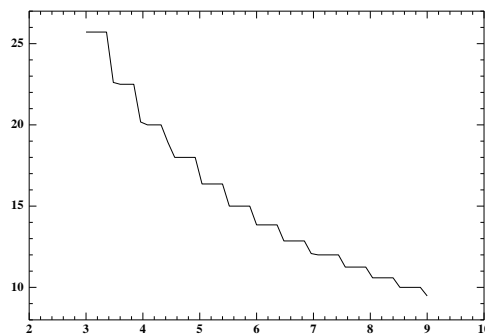
Figure 4.9 \delta\phi = f\left(\frac{D}{\lambda_{min}} \sin \theta_{max}\right) à l'optimum
