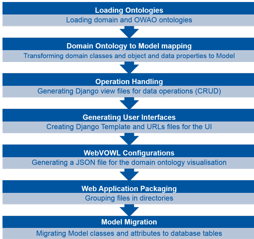
Figure 4.2: GenAppi generator workflow.
