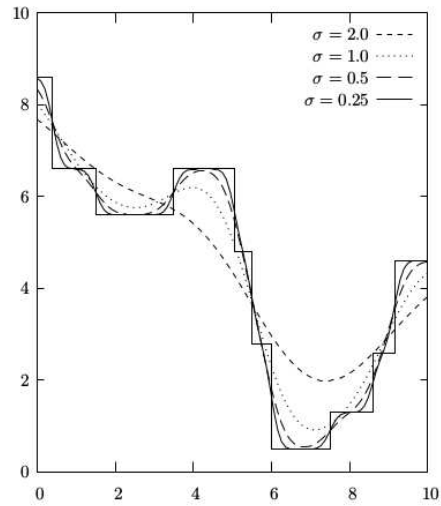
Figure 2.7: Example of different smoothing operators on \mathcal{L}_f
