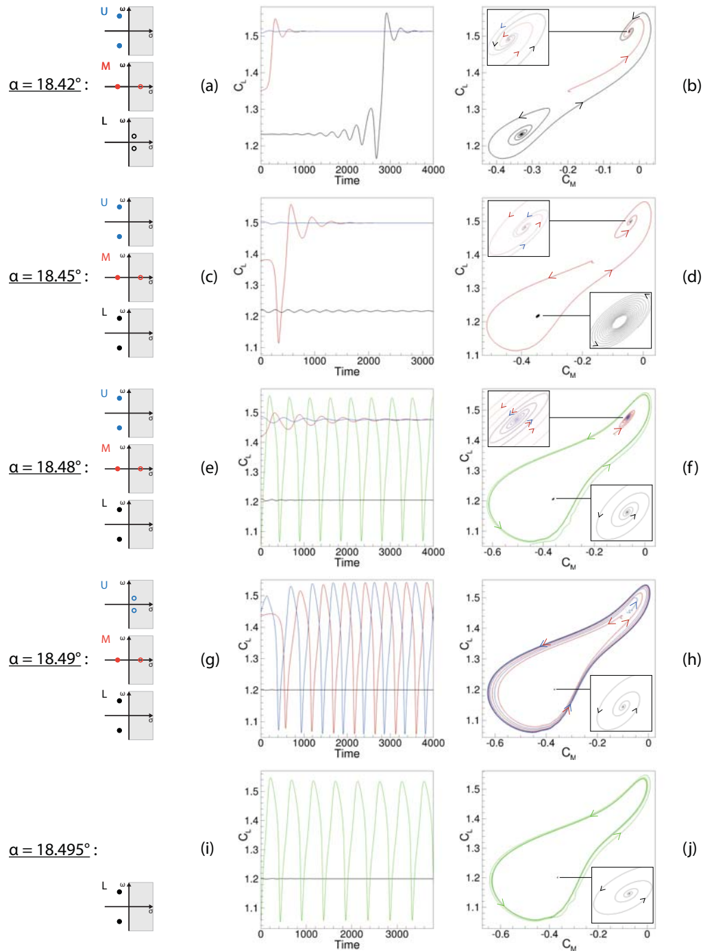
FIGURE 6.7: Temporal solutions represented in two different planes ( t, C_L ) (left pictures) and (C_M, C_L) (right pictures, also often called phase portrait) for different initial conditions and angles of attack. (a) and (b): \alpha = 18.42^\circ . (c) and (d): \alpha = 18.45^\circ . (e) and (f): \alpha = 18.48^\circ . (g) and (h): \alpha = 18.49^\circ . (i) and (j): \alpha = 18.495^\circ . For each angle of attack, the color of the curve refers to the color of the cross in Figure (6.6)(b), marking the solution used to initialize the unsteady computation indicated. The linear behavior of the steady solutions is recalled next to the temporal solutions, as well as the angles of attack.
