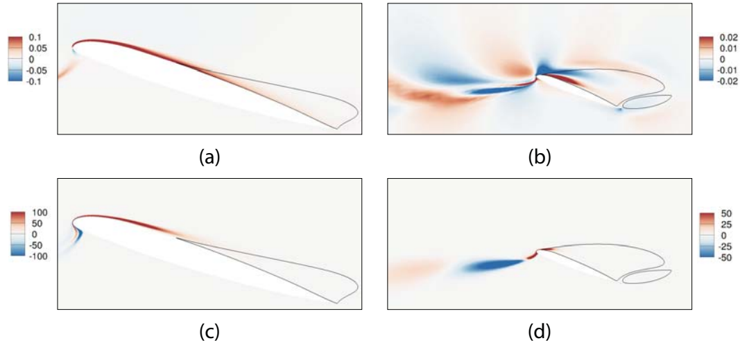
FIGURE 5.9: Visualisation of the structure of the adjoint modes. (a) Real part of the \rho u^\dagger field of the stall adjoint mode ( \alpha = 18.49^\circ ). (c) Real part of the \rho v^\dagger field of the stall adjoint mode ( \alpha = 18.49^\circ ). (b) Real part of the \rho u^\dagger field of the vortex-shedding eigenmode ( \alpha = 21.00^\circ ). (d) Real part of the \rho v^\dagger field of the vortex-shedding eigenmode ( \alpha = 21.00^\circ ).
