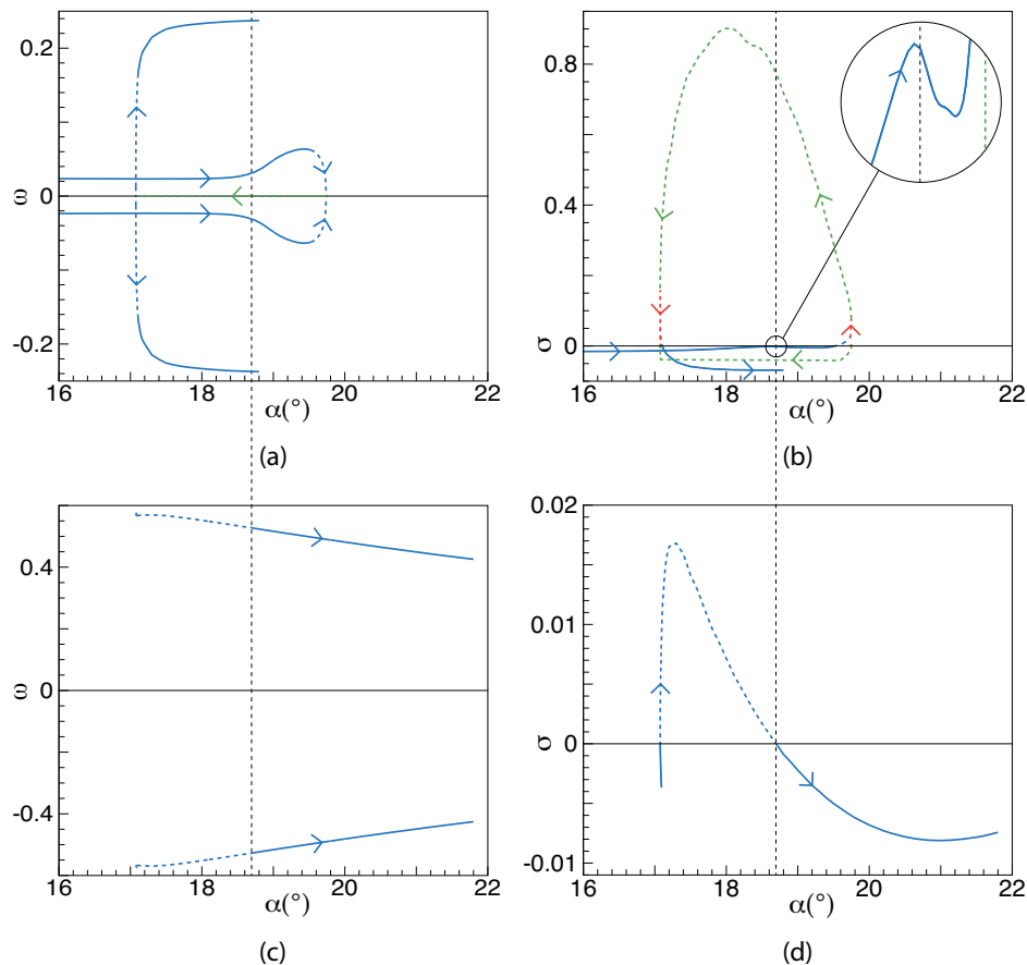
FIGURE 8.15: Evolution of the eigenvalues as a function of the angle of attack in the case of a NACA0012 at \text{Re} = 1.0 \times 10^6 with the Edwards–Chandra modification of the Spalart–Allmaras model. (a) and (c): evolution of the angular frequency as a function of the angle of attack. (b) and (d): evolution of the growth rate as a function of the angle of attack. (a) and (b): stall mode. (c) and (d): vortex shedding mode. The direction of the arrows refers to increasing curvilinear abscissa.
