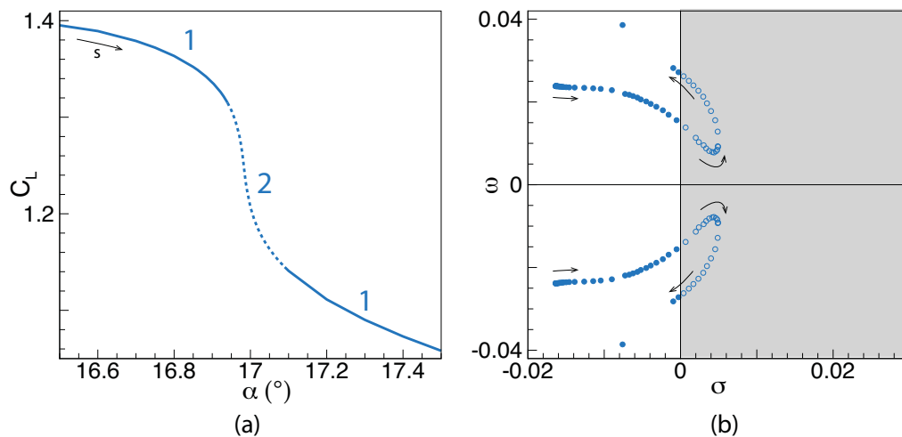
FIGURE 8.2: Real evolution of the temporal behavior of the leading mode. (a) polar curve zoomed in close to stall and associated temporal behavior. (b) Superimposition of the spectra obtained from each steady solution along the polar curve (the black arrows indicate the direction of an increasing curvilinear abscissa). The color code is similar to the one of Figure (7.17) in chapter 7. The grey area corresponds to the zone in which the modes are unstable.
