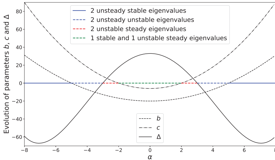
FIGURE E.2: Representation of the steady state c_{l_0} = 0 with the linear behavior associated for each value of \alpha (see associated color code in legend). This linear behavior is based on the evolution of parameters b , c and \delta also plotted. Every time that one of these parameters changes of sign, the linear behavior of the steady state evolves (as described in Table E.2. b is represented with a factor 8 and c with a factor 3 for visualization purpose.
