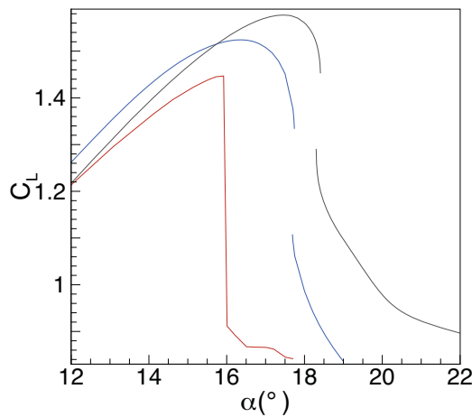
FIGURE 3.6: Comparison of the evolution of the lift coefficient as a function of the angle attack for a two dimensional OA209 airfoil at Re = 1.8 \times 10^6 . Red curve: experimentally (from Le Pape et al. [125]). Blue curve: numerically from steady RANS solutions with the k - \omega model (from Richez et al. [133]). Black curve: numerically from steady RANS solutions with the Spalart–Allmaras model (from the present study).
