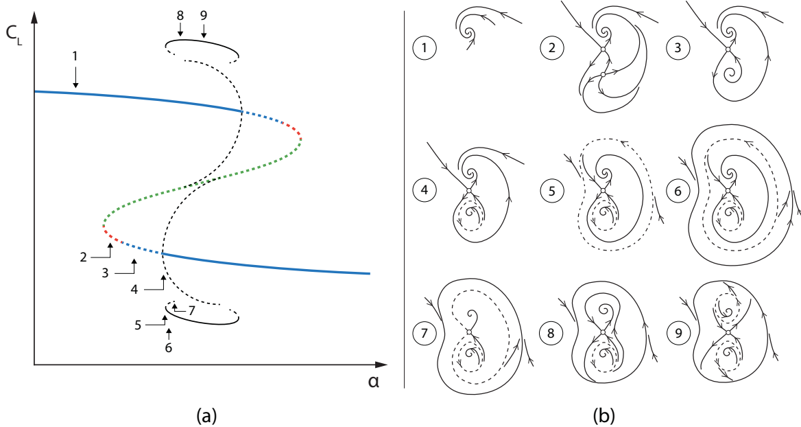
FIGURE 7.13: Second stall scenario. Same legend as in Figure (7.12).
