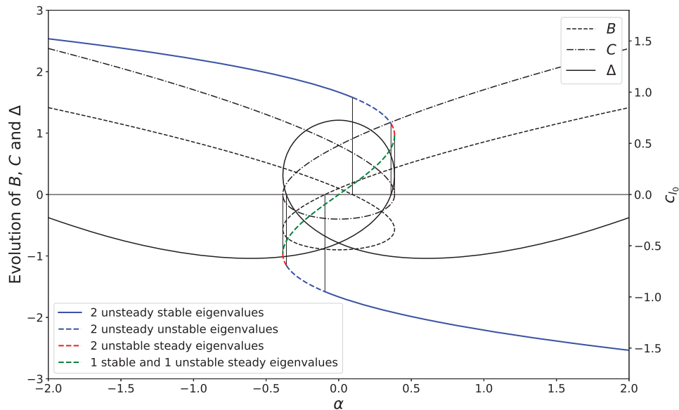
FIGURE E.3: Representation of the steady state c_{l_0} as a function of \alpha with the linear behavior associated for each value of \alpha (see associated color code in legend). This linear behavior is based on the evolution of parameters B , C and \Delta also plotted. Every time that one of these parameters changes of sign, the linear behavior of the steady state evolves (as described in Table (E.2)). Similar to Figure (E.2) but with non-null steady states and parameters B , C and \Delta functions of the steady states.
