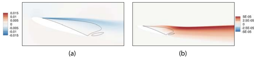
FIGURE 8.10: Visualisation of the structure of the eigenmodes. (a) Real part of the \hat{\rho}u field of the stall eigenmode ( \alpha = 18.05^\circ ). (b) Real part of the \hat{\rho}v field of the stall eigenmode ( \alpha = 18.05^\circ ).
