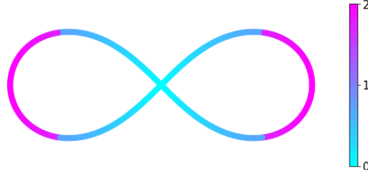
Figure IV.5: Values of the normal reach on the lemniscate of Bernoulli.
