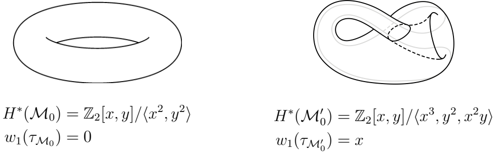
Figure I.26: The cohomology rings of \mathcal{M}_0 and \mathcal{M}'_0 over \mathbb{Z}_2 , and the first Stiefel-Whitney classes of their respective tangent bundles \tau_{\mathcal{M}_0} and \tau_{\mathcal{M}'_0} .
