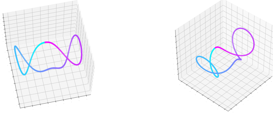
Figure I.22: Two views of the submanifold \check{\mathcal{M}} \subset \mathbb{R}^2 \times \mathbf{M}(\mathbb{R}^2) , projected in a 3-dimensional subspace via PCA. Observe that it does not self-intersect. The initial set \mathcal{M} is represented in Figure I.21.
