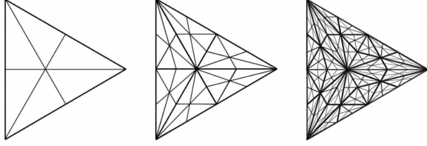
Figure II.3: The first three barycentric subdivisions of a 2-simplex.
