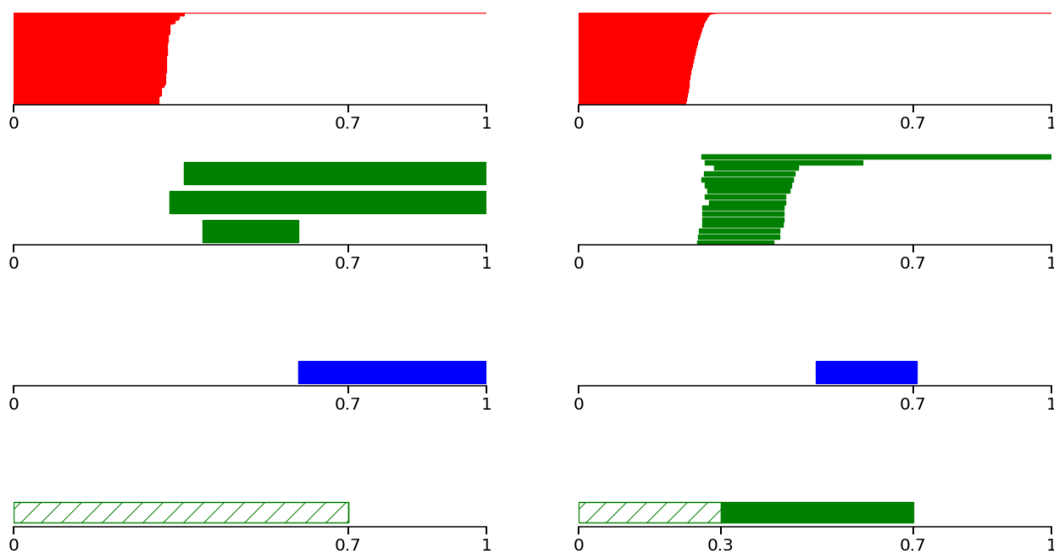
Figure V.12: Left: H^0 , H^1 and H^2 barcodes of X and lifebar of w_1(X) . Right: same for X' .
