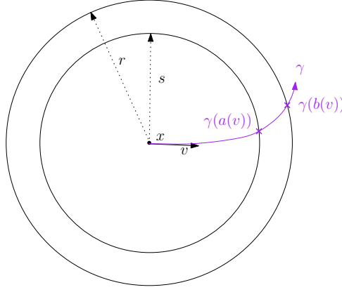
Figure IV.11: Illustration of a(v) and b(v) in the proof of Proposition IV.16.
