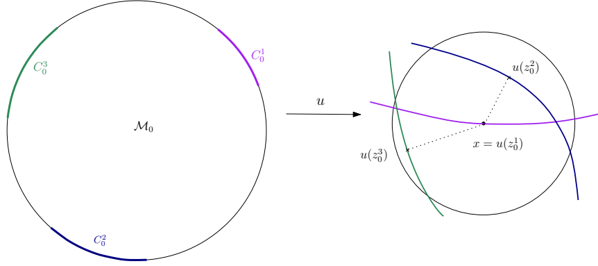
Figure IV.23: The connected components C_0^i .
