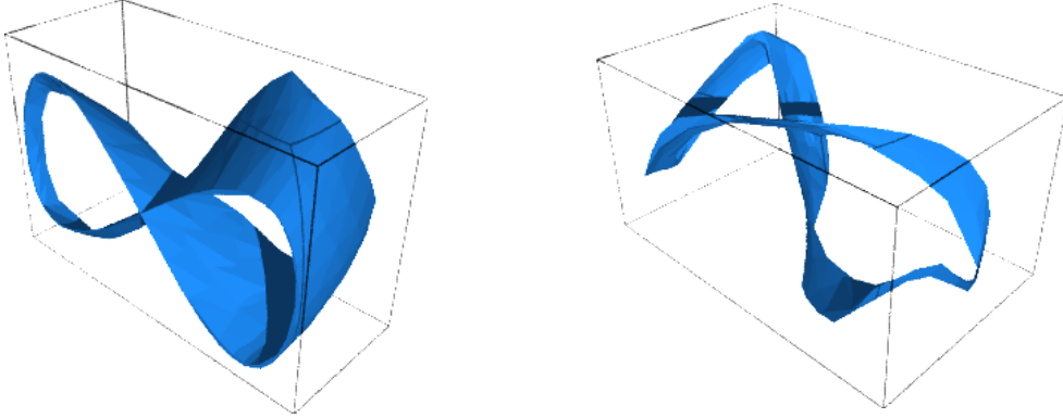
Figure IV.18: Left: A section of \mathcal{M} . Right: The corresponding section of \tilde{\mathcal{M}} , projected in a 3-dimensional subspace via PCA. Observe that it does not self-intersect.
