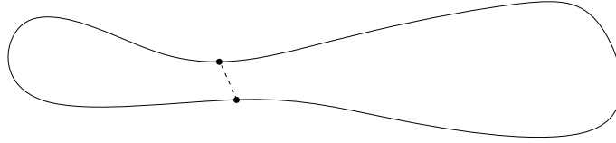
Figure IV.2: Pair of points for which the geodesic distance is large compared to the Euclidean distance.
