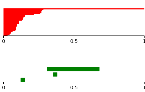
A persistence barcode
