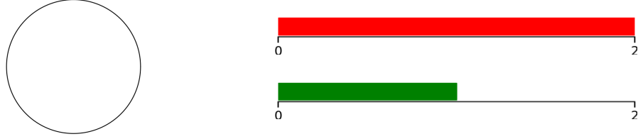
Figure II.6: Example for t^\circ = t^\bullet . Left: the set \mathcal{M} . Right: Barcode (V[\mathcal{M}]) .
