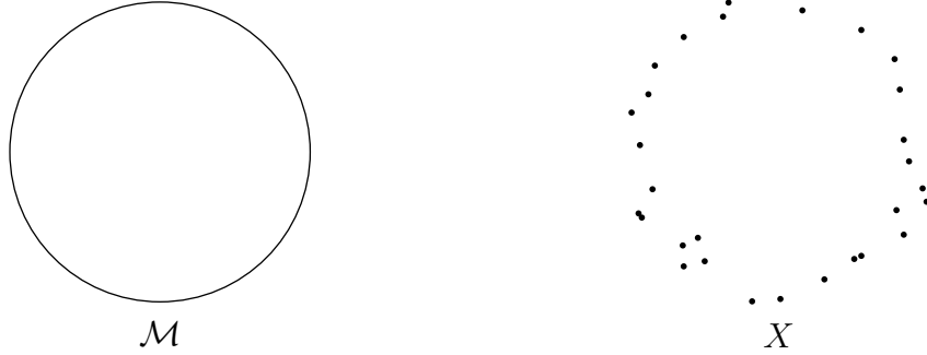
Figure I.17: The underlying space and the observation.
