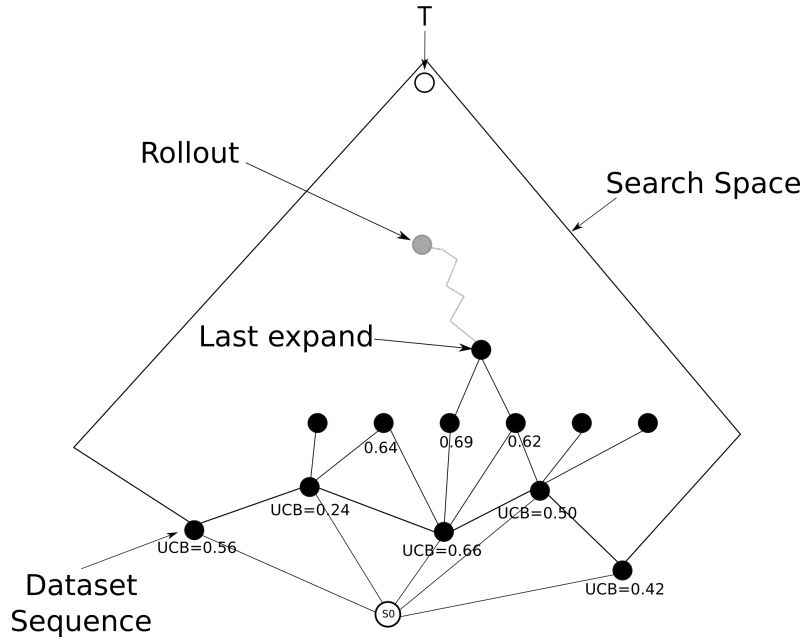
Рис. 4.3: MCTSExtent Principle.
