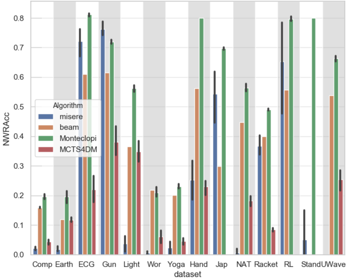
Рис. 5.2: Mean NWRAcc of top-5 patterns with different algorithms. Bar errors represent the 95% confidence intervals
