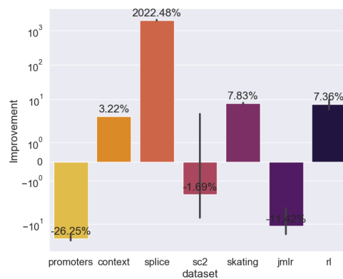
Рис. 4.8: SeqScout vs. Beam Search
