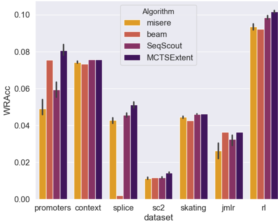
FIG. 4.6: Mean WRAcc of top-5 best patterns (10K iterations)
