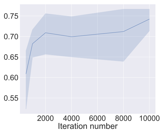
Рис. 6.11: Accuracy w.r.t. the number of iterations
