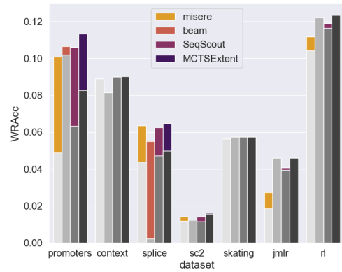
Рис. 4.25: Added value of local optima search for 10,000 iterations
