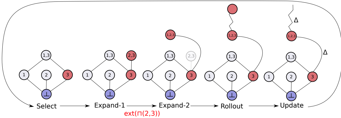
Рис. 5.1: Simple illustration of MonteCloPi steps
