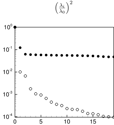
Figure 2.11: Separation of Singular-Values (\lambda_i/\lambda_0)^2 for the \tilde{\mathbf{f}}_{\mathbf{x}} model 1 (black dots) and the \tilde{f}_{\tilde{v}} model 2 (white dots), computed around the RANS-SA solution.
