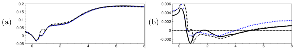
Figure 3.9: Wall-pressure assimilation: wall-pressure (a) and wall-friction (b) for models 1 and 2.
