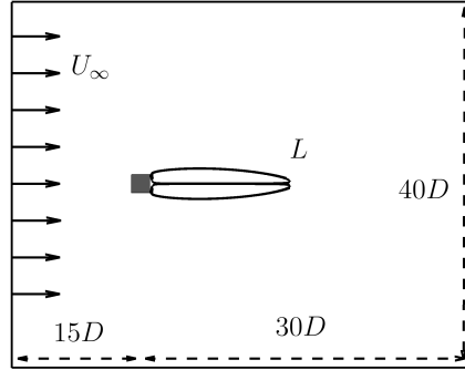
Figure 4.1: Sketch of the physical domain and inflow boundary condition for the square cylinder case. The re-circulation bubble’s length is indicated in the figure and will be defined as L .
