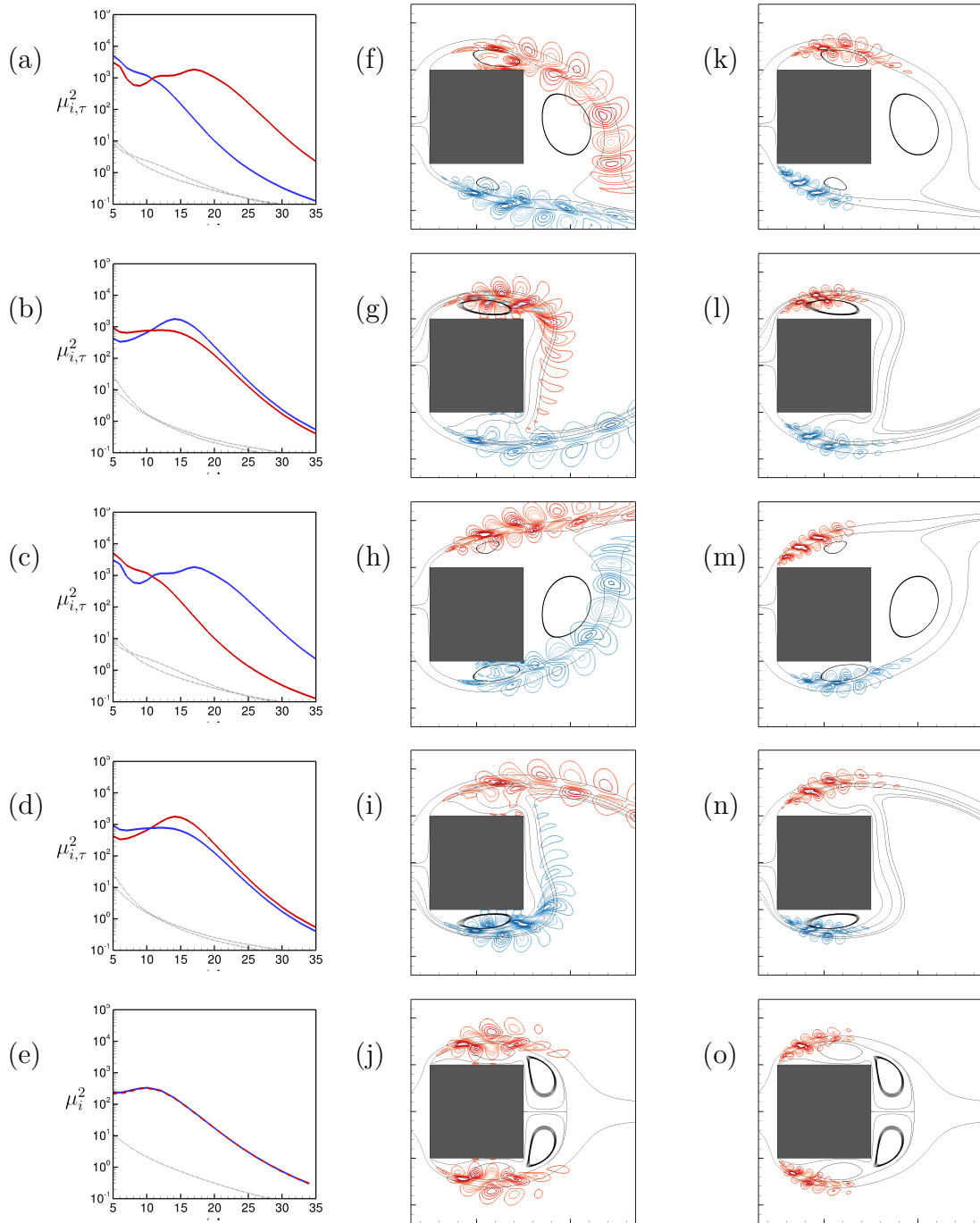
Figure 5.7: Resolvent analysis for the broadband high-frequency component. Quasi-static approximation (a,b,c,d) for \tau/T = 0 (a), 1/4 (b), 2/4 (c) and 3/4 (d): upper/lower modes Resolvent gains (first column) and their respective modes at \omega = 10 (second column) and \omega = 20 (third column). Red and blue modes correspond to upper/lower modes. (e) Steady-flow approximation: optimal/sub-optimal gains (first column) and leading modes for \omega = 10 (second column) and \omega = 20 (third column).
