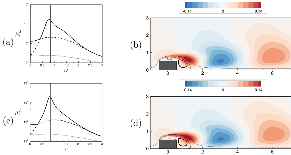
Figure 6.3: Resolvent Analysis on (URANS) mean-flow: optimal (thick lines) and sub-optimal gains (dashed lines) and leading mode at \omega = 0.83 (grey vertical line) for (a,b) frozen \nu_t and (c,d) variable \nu_t .
