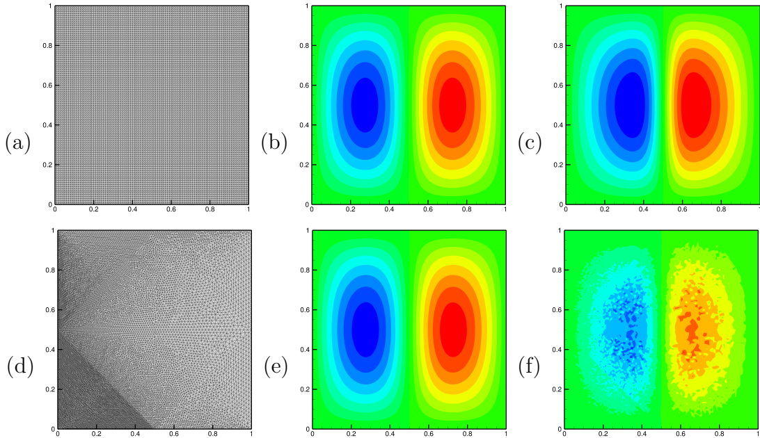
Figure B.2: Discrete Formalism Optimization: mesh (a,d), optimal solution u^* (b,e) and optimal forcing term f^* (c,f).
