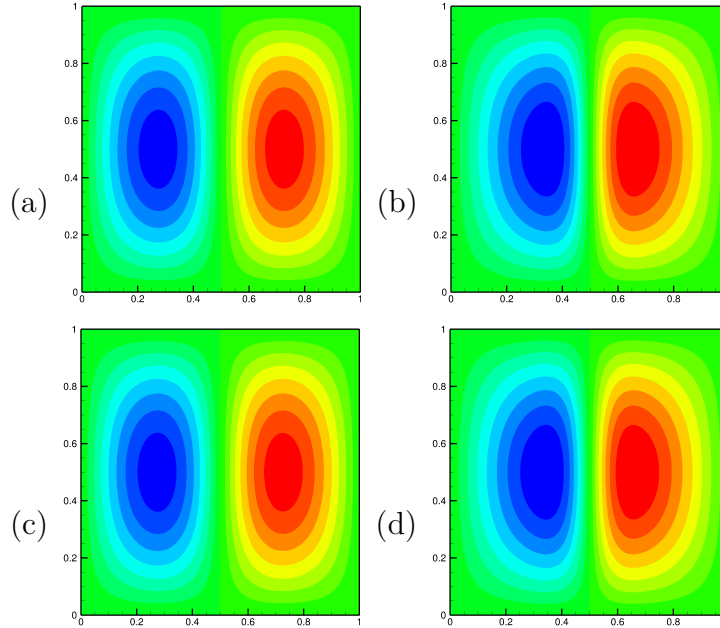
Figure B.4: Cholesky decomposition change of variables: final solution (a,c) and forcing term (b,d) for meshes 1 (a,b) and 2 (c,d).
