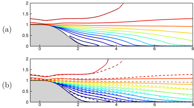
Figure 2.6: Complete velocity field assimilation: optimal velocity field when optimizing (a) \tilde{\mathbf{f}}_{\mathbf{x}} (model 1) and (b) \tilde{f}_{\tilde{\nu}} (model 2). The reference (DNS) is provided in dashed lines in both plots.
