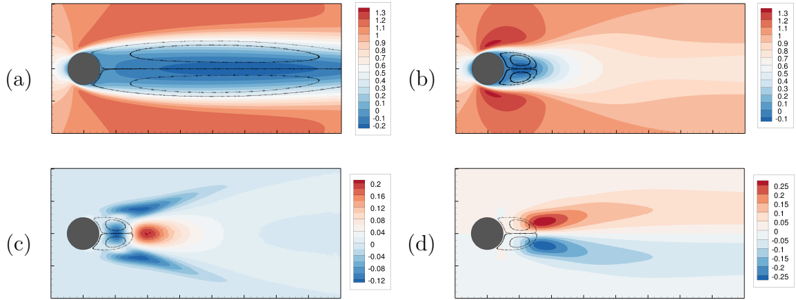
Figure 3.1: (a) Unstable steady-state (longitudinal velocity) solution and also the starting point of our optimization procedure and (b) mean-flow and exact divergence Reynolds-stress tensor \bar{f}_x, \bar{f}_y (c,d)
