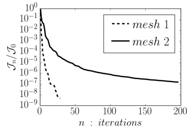
Figure B.3: Discrete Formalism Optimization: Convergence of the cost functional \mathcal{J}_n/\mathcal{J}_0 .
