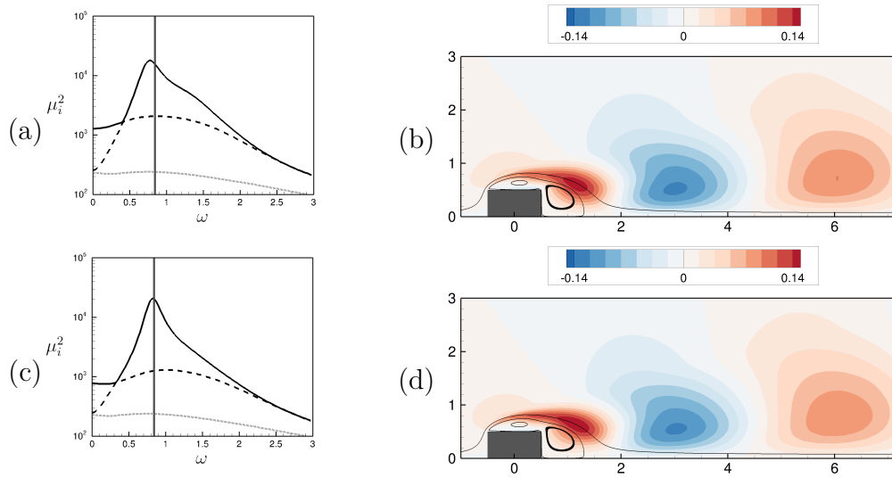
Figure 6.3: resolvent Analysis on (URANS) mean-flow: gains and leading mode at \omega = 0.83 (grey vertical line) for (a,b) frozen \nu_t and (c,d) variable \nu_t .
