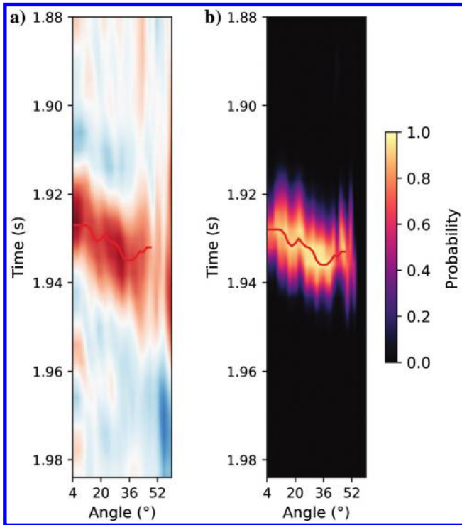
Figure 11. Prediction of the top reservoir across the prestack domain. (a) Angle gather at inline 27208 and crossline 16022; the predicted horizon is drawn in red. The prediction is following the moveout of the reflector up to 40°, and it fails to recognize the event once the waveform becomes too different from the reference near stack, in particular because of stretching. (b) Prediction probability.
