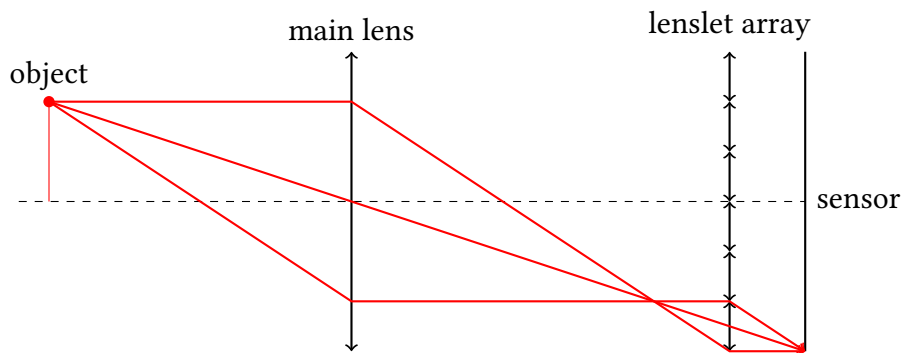
Figure 1.14: Optical configuration of a plenoptic camera 2.0
