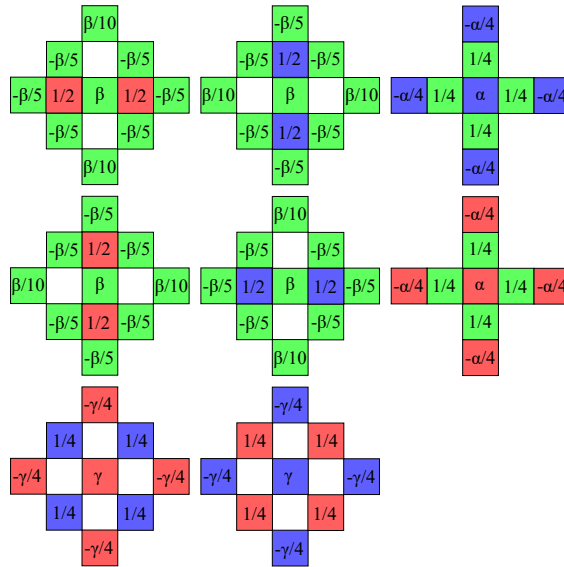
Figure 2.2: Kernels in [42]
