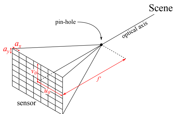
Figure 1.16: Pinhole model
