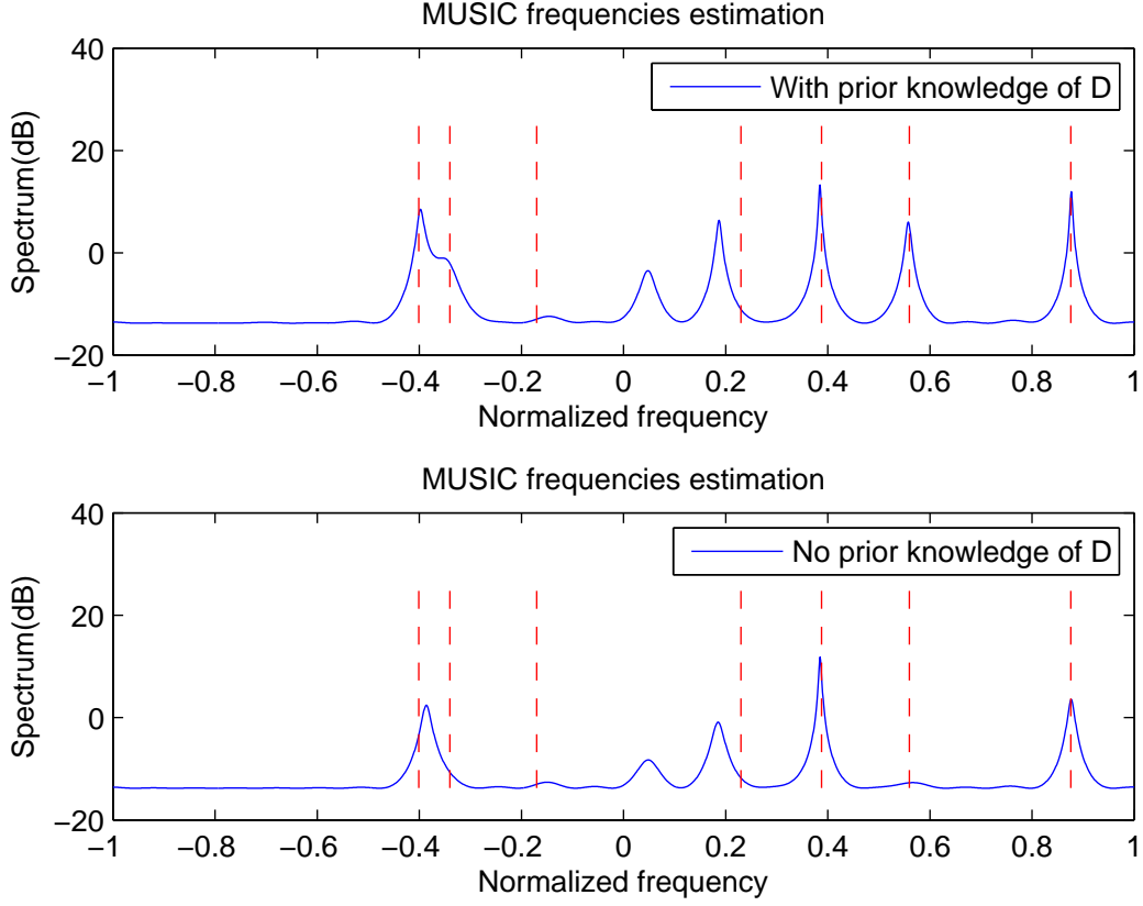
Figure 2.5 – MUSIC spectrum with coprime sampling in the diagonal property loss condition, 7 sinusoidal components, M = 4 and N = 5 .
