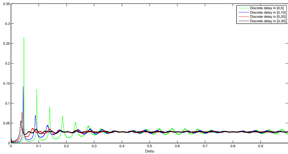
Figure 2.4 – Statistical mean of (2.18) versus different values of \Delta , \alpha satisfies discrete uniform distribution, distributed in range [0,5],[0,10],[0,20],[0,30] . M = 4, N = 5 .
