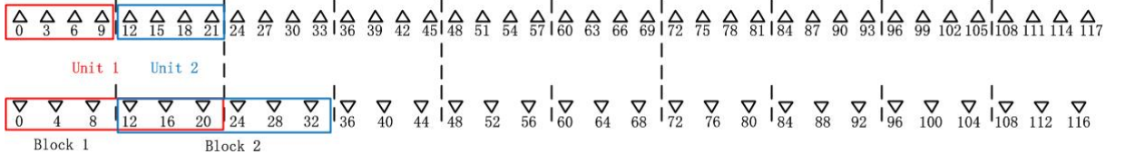
Figure 1.4 – Collected samples of two samplers with M = 3, N = 4 .
