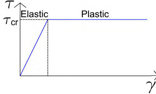
Figure 2-8: Elasto-plastic behavior of the coating layer.
